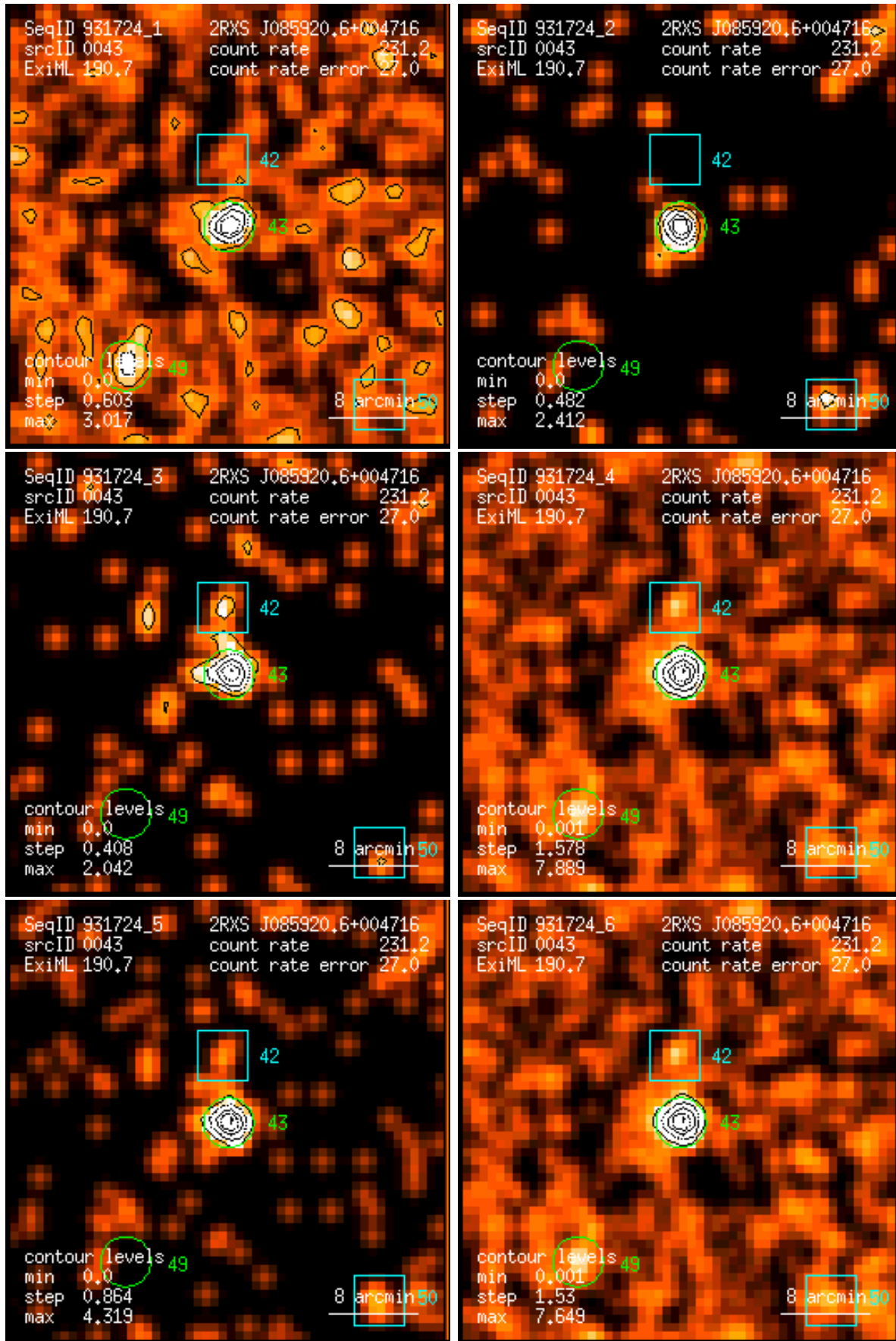
Figure 43: RASS 931724: detection 0043: band rate images, Gaussian filter: (1) PSPC channels 11 – 41, (2) 52 – 90, (3) 91 – 201, (4) 11 – 235, (5) 52 – 201, (6) 11 – 201. Broad band rates in counts/ks. Band rate contour levels in counts/ks/arcmin 2 .
