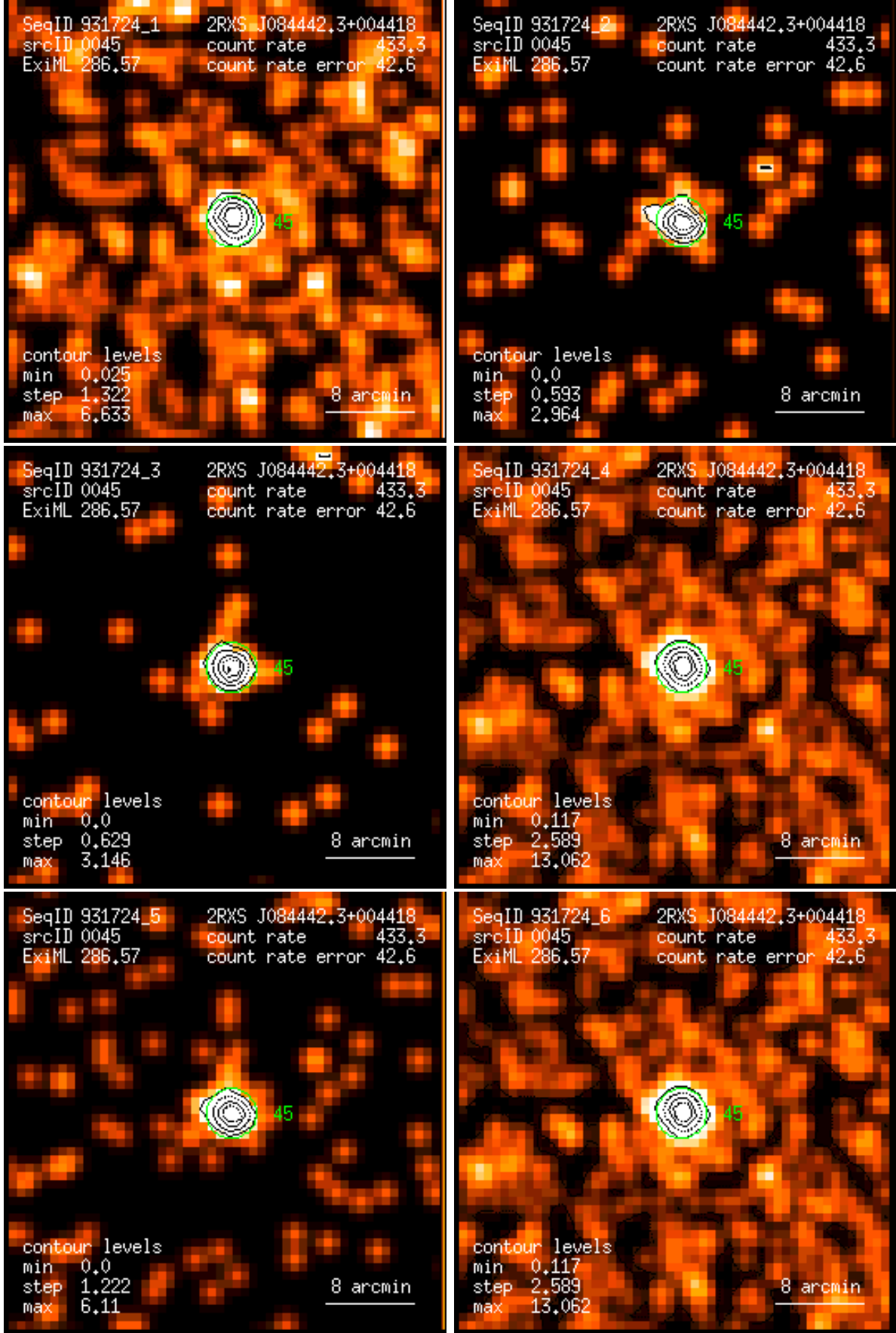
Figure 45: RASS 931724: detection 0045: band rate images, Gaussian filter: (1) PSPC channels 11 – 41, (2) 52 – 90, (3) 91 – 201, (4) 11 – 235, (5) 52 – 201, (6) 11 – 201. Broad band rates in counts/ks. Band rate contour levels in counts/ks/arcmin 2 .
