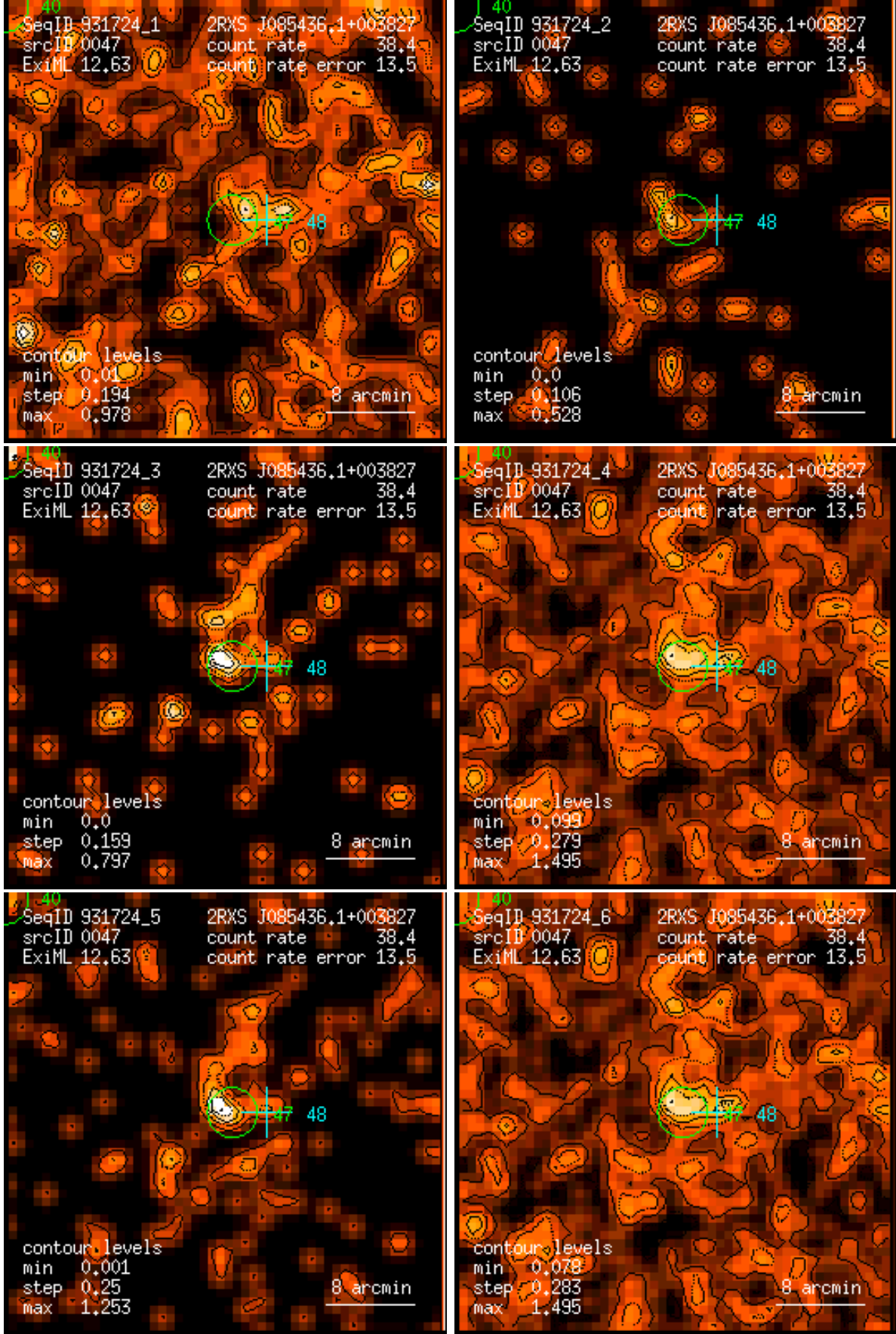
Figure 47: RASS 931724: detection 0047: band rate images, Gaussian filter: (1) PSPC channels 11 – 41, (2) 52 – 90, (3) 91 – 201, (4) 11 – 235, (5) 52 – 201, (6) 11 – 201. Broad band rates in counts/ks. Band rate contour levels in counts/ks/arcmin 2 .
