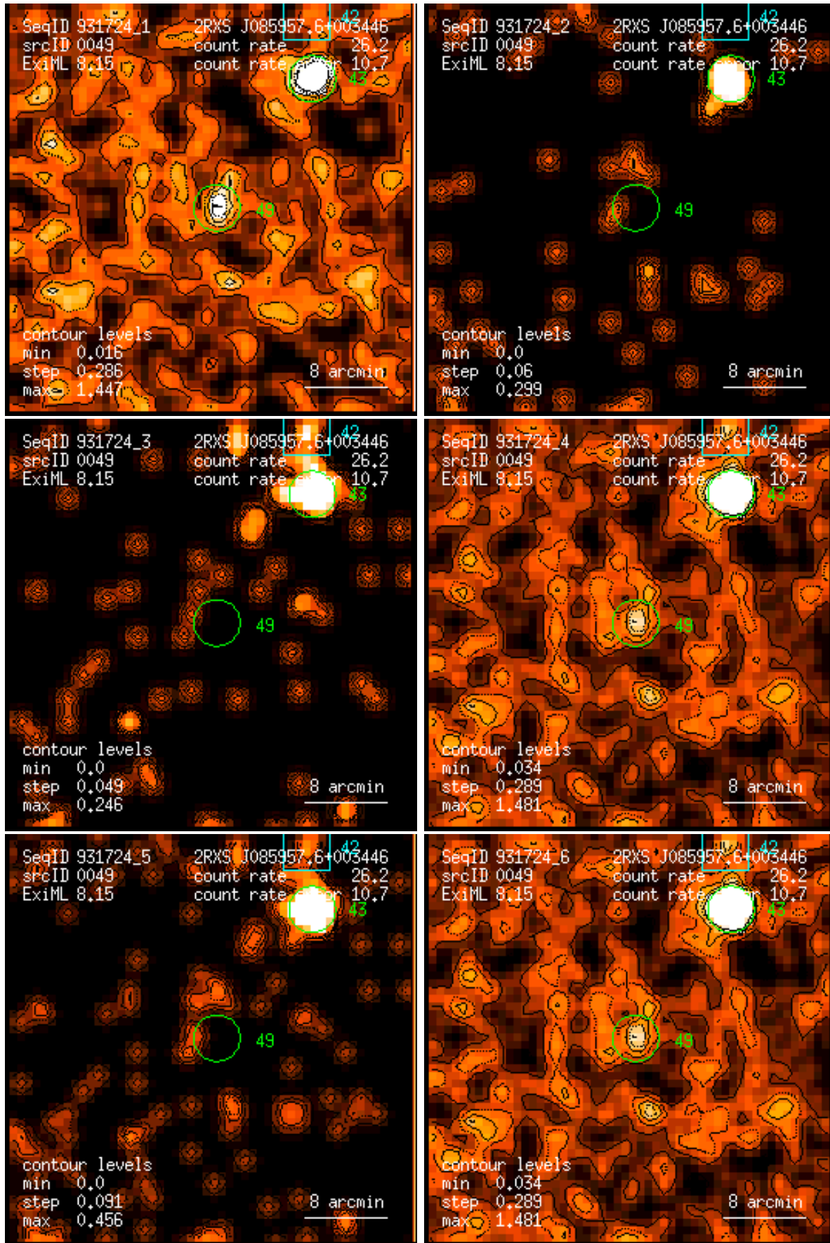
Figure 49: RASS 931724: detection 0049: band rate images, Gaussian filter: (1) PSPC channels 11 – 41, (2) 52 – 90, (3) 91 – 201, (4) 11 – 235, (5) 52 – 201, (6) 11 – 201. Broad band rates in counts/ks. Band rate contour levels in counts/ks/arcmin 2 .
