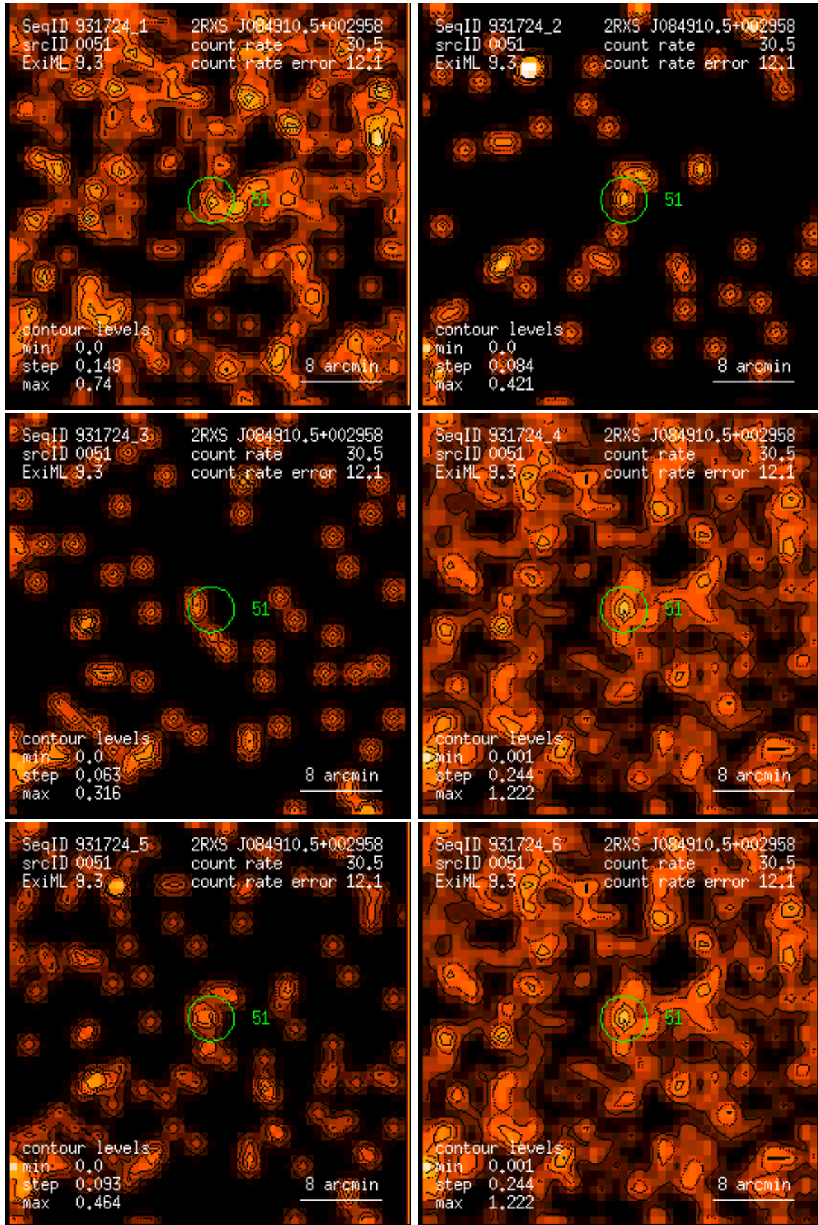
Figure 51: RASS 931724: detection 0051: band rate images, Gaussian filter: (1) PSPC channels 11 – 41, (2) 52 – 90, (3) 91 – 201, (4) 11 – 235, (5) 52 – 201, (6) 11 – 201. Broad band rates in counts/ks. Band rate contour levels in counts/ks/arcmin 2 .
