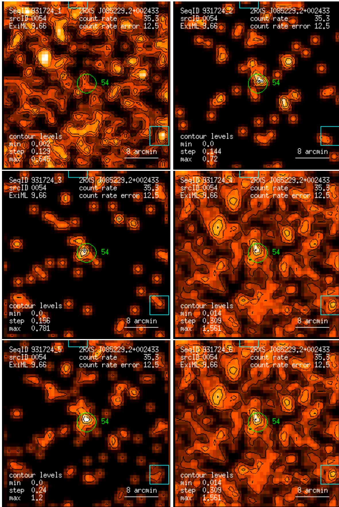
Figure 54: RASS 931724: detection 0054: band rate images, Gaussian filter: (1) PSPC channels 11 – 41, (2) 52 – 90, (3) 91 – 201, (4) 11 – 235, (5) 52 – 201, (6) 11 – 201. Broad band rates in counts/ks. Band rate contour levels in counts/ks/arcmin 2 .
