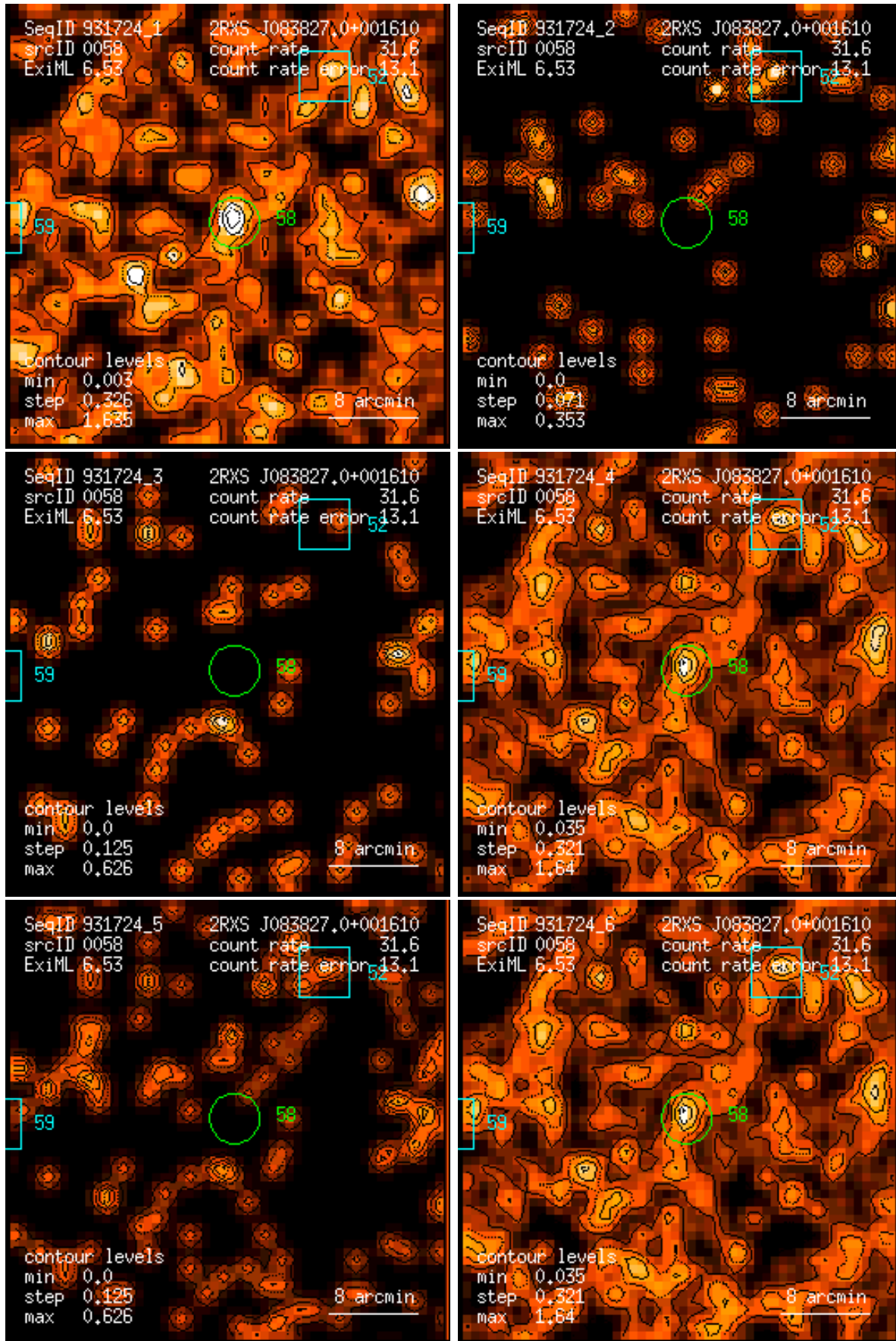
Figure 58: RASS 931724: detection 0058: band rate images, Gaussian filter: (1) PSPC channels 11 – 41, (2) 52 – 90, (3) 91 – 201, (4) 11 – 235, (5) 52 – 201, (6) 11 – 201. Broad band rates in counts/ks. Band rate contour levels in counts/ks/arcmin 2 .
