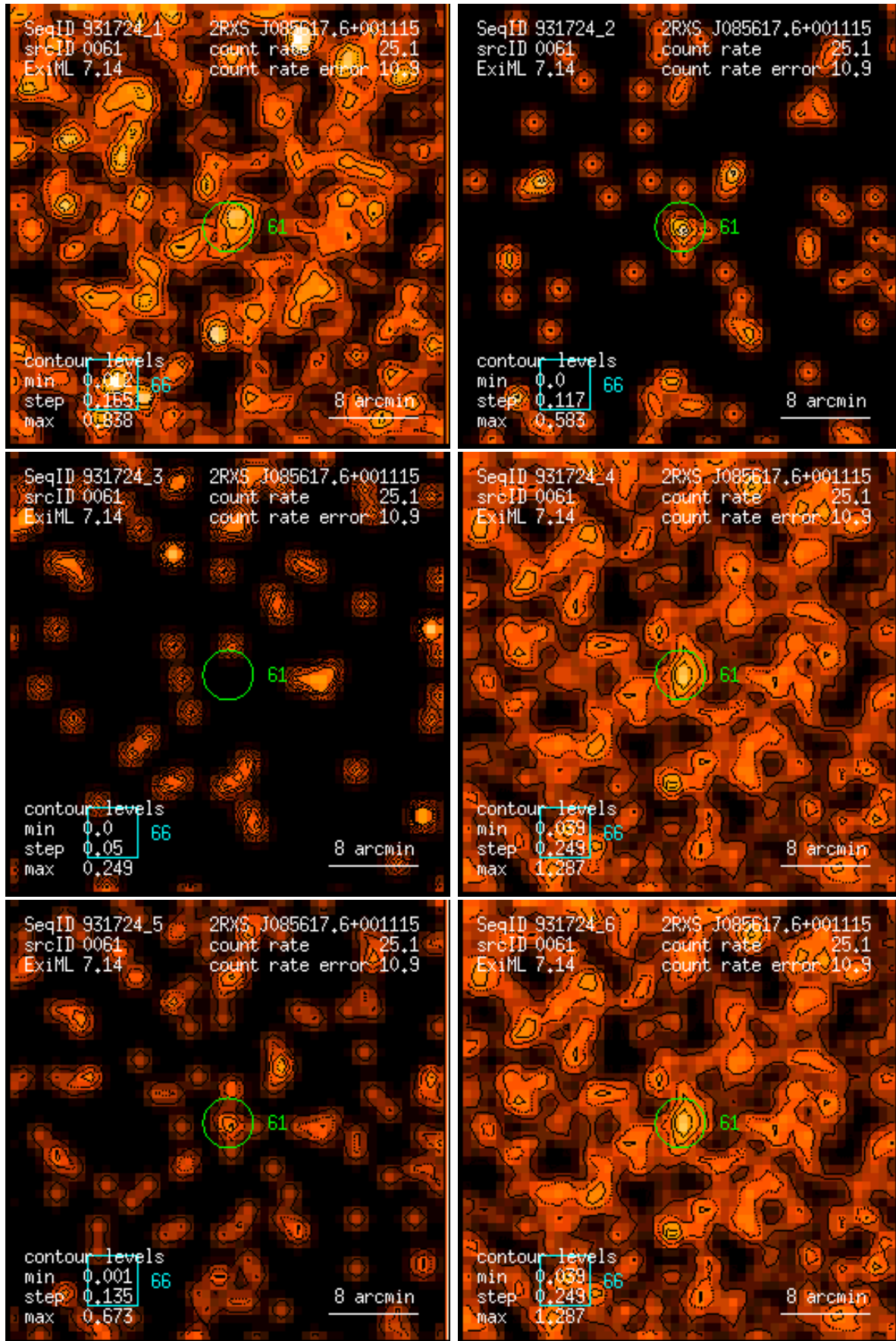
Figure 61: RASS 931724: detection 0061: band rate images, Gaussian filter: (1) PSPC channels 11 – 41, (2) 52 – 90, (3) 91 – 201, (4) 11 – 235, (5) 52 – 201, (6) 11 – 201. Broad band rates in counts/ks. Band rate contour levels in counts/ks/arcmin 2 .
