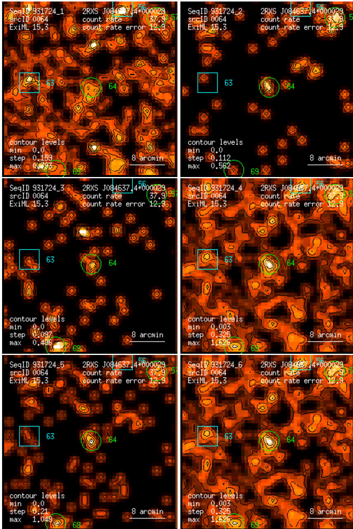
Figure 64: RASS 931724: detection 0064: band rate images, Gaussian filter: (1) PSPC channels 11 – 41, (2) 52 – 90, (3) 91 – 201, (4) 11 – 235, (5) 52 – 201, (6) 11 – 201. Broad band rates in counts/ks. Band rate contour levels in counts/ks/arcmin 2 .
