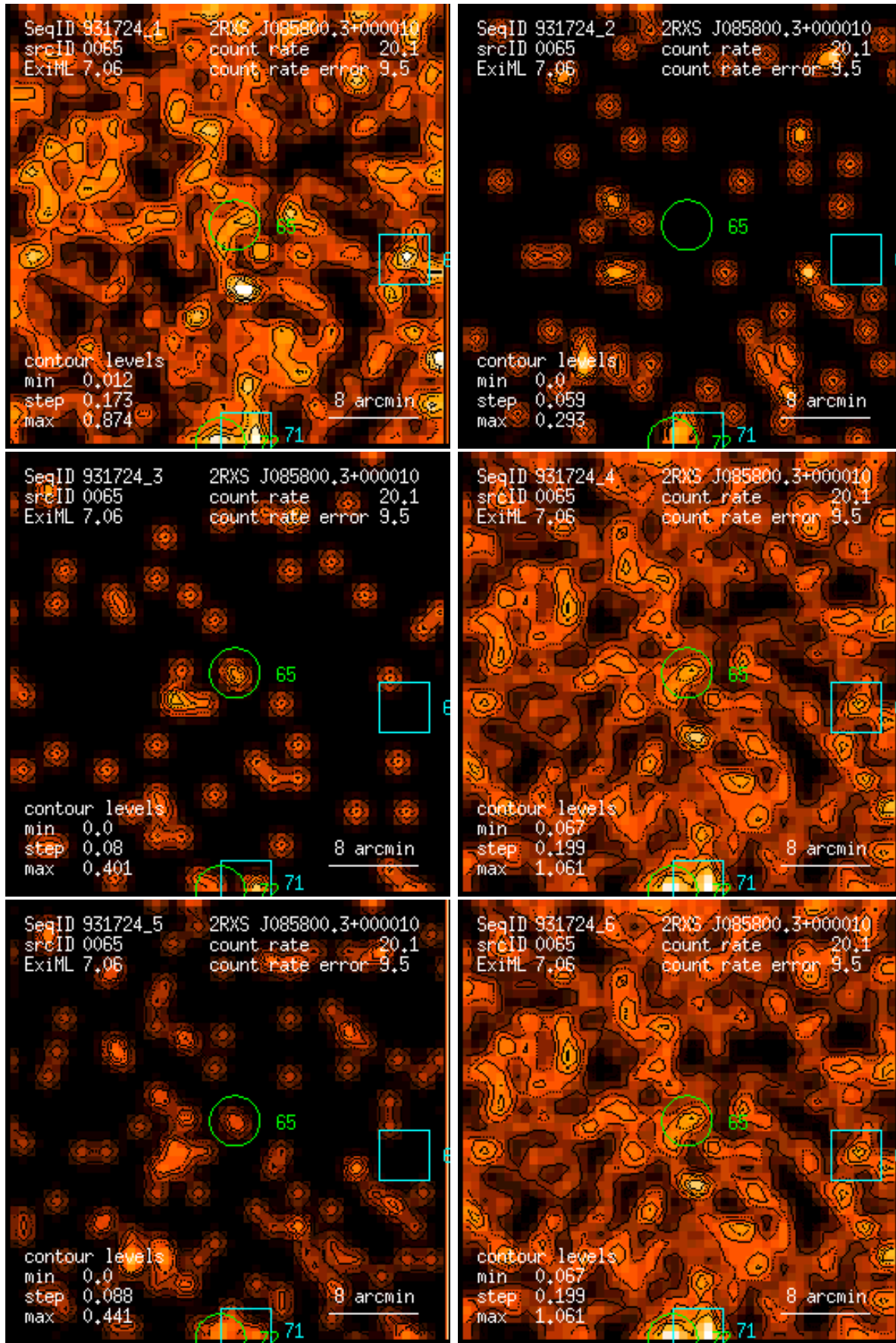
Figure 65: RASS 931724: detection 0065: band rate images, Gaussian filter: (1) PSPC channels 11 – 41, (2) 52 – 90, (3) 91 – 201, (4) 11 – 235, (5) 52 – 201, (6) 11 – 201. Broad band rates in counts/ks. Band rate contour levels in counts/ks/arcmin 2 .
