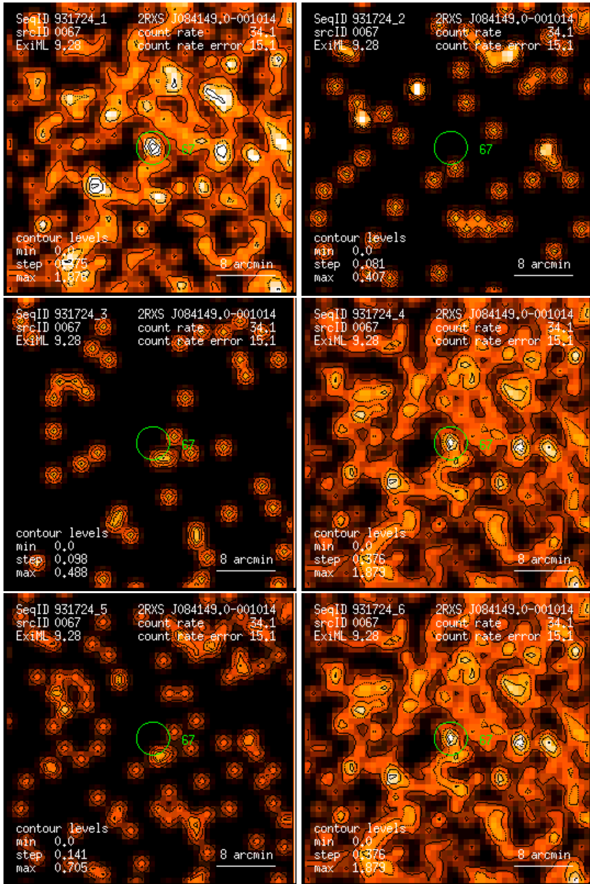
Figure 67: RASS 931724: detection 0067: band rate images, Gaussian filter: (1) PSPC channels 11 – 41, (2) 52 – 90, (3) 91 – 201, (4) 11 – 235, (5) 52 – 201, (6) 11 – 201. Broad band rates in counts/ks. Band rate contour levels in counts/ks/arcmin 2 .
