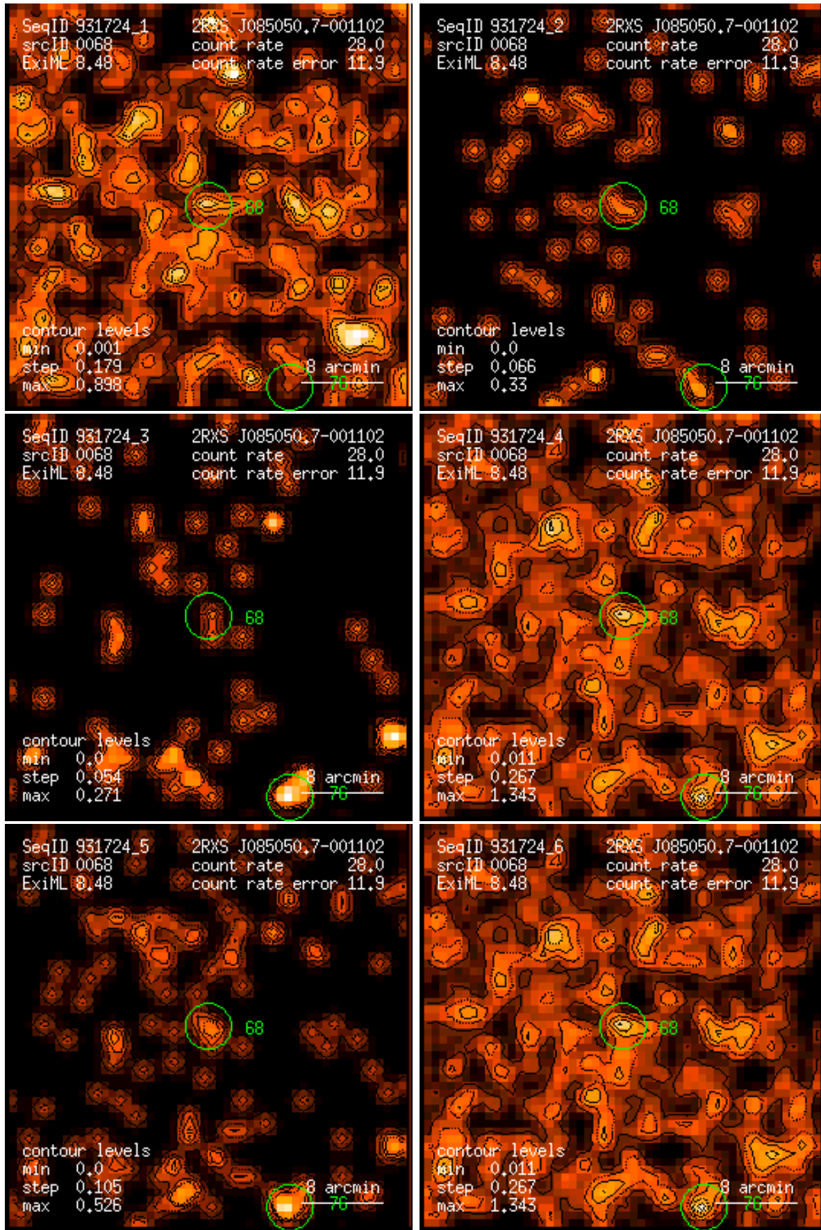
Figure 68: RASS 931724: detection 0068: band rate images, Gaussian filter: (1) PSPC channels 11 – 41, (2) 52 – 90, (3) 91 – 201, (4) 11 – 235, (5) 52 – 201, (6) 11 – 201. Broad band rates in counts/ks. Band rate contour levels in counts/ks/arcmin 2 .
