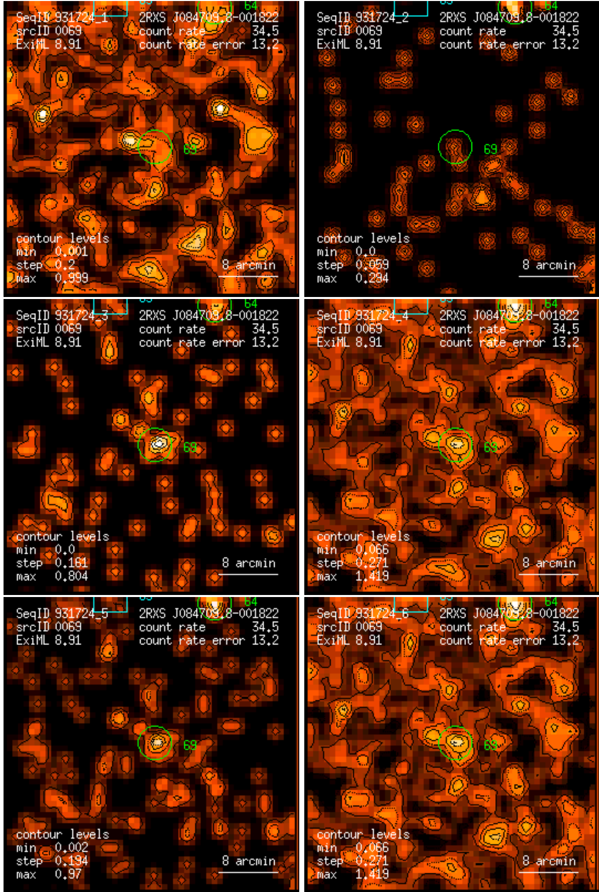
Figure 69: RASS 931724: detection 0069: band rate images, Gaussian filter: (1) PSPC channels 11 – 41, (2) 52 – 90, (3) 91 – 201, (4) 11 – 235, (5) 52 – 201, (6) 11 – 201. Broad band rates in counts/ks. Band rate contour levels in counts/ks/arcmin 2 .
