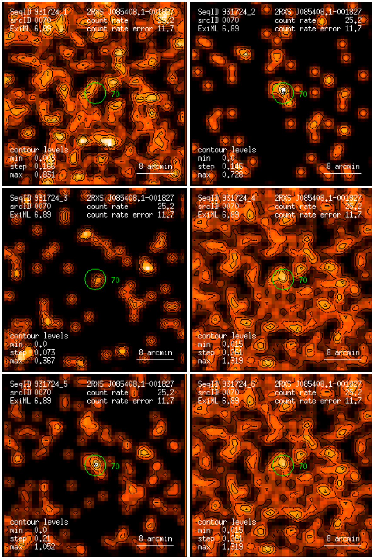
Figure 70: RASS 931724: detection 0070: band rate images, Gaussian filter: (1) PSPC channels 11 – 41, (2) 52 – 90, (3) 91 – 201, (4) 11 – 235, (5) 52 – 201, (6) 11 – 201. Broad band rates in counts/ks. Band rate contour levels in counts/ks/arcmin 2 .
