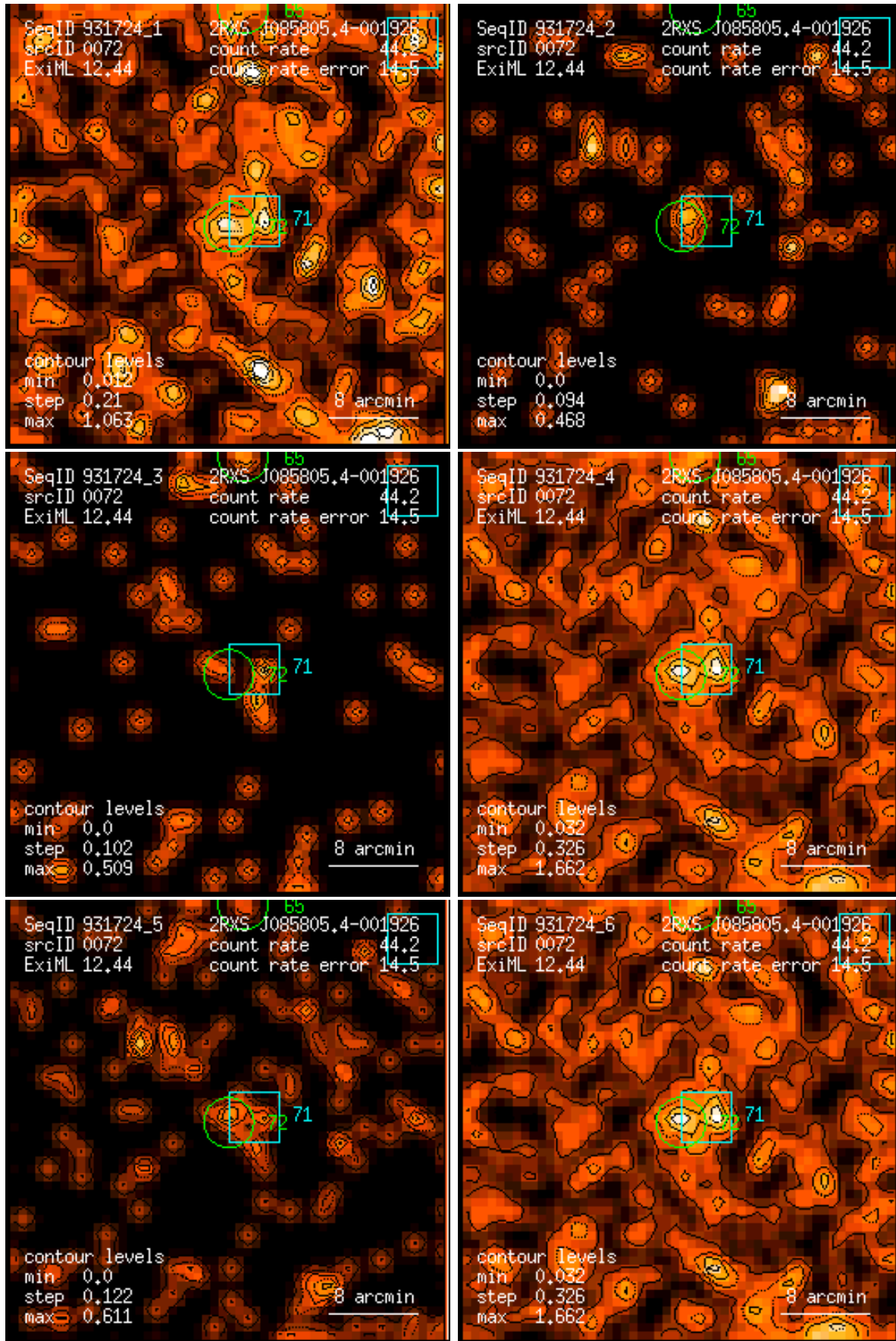
Figure 72: RASS 931724: detection 0072: band rate images, Gaussian filter: (1) PSPC channels 11 – 41, (2) 52 – 90, (3) 91 – 201, (4) 11 – 235, (5) 52 – 201, (6) 11 – 201. Broad band rates in counts/ks. Band rate contour levels in counts/ks/arcmin 2 .
