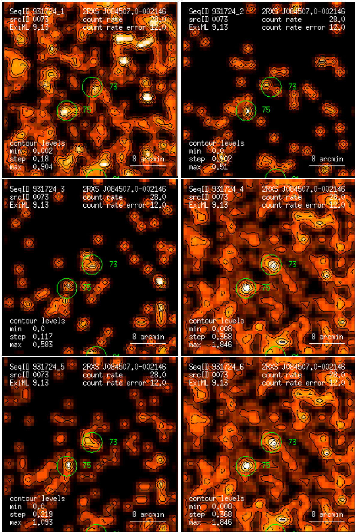
Figure 73: RASS 931724: detection 0073: band rate images, Gaussian filter: (1) PSPC channels 11 – 41, (2) 52 – 90, (3) 91 – 201, (4) 11 – 235, (5) 52 – 201, (6) 11 – 201. Broad band rates in counts/ks. Band rate contour levels in counts/ks/arcmin 2 .
