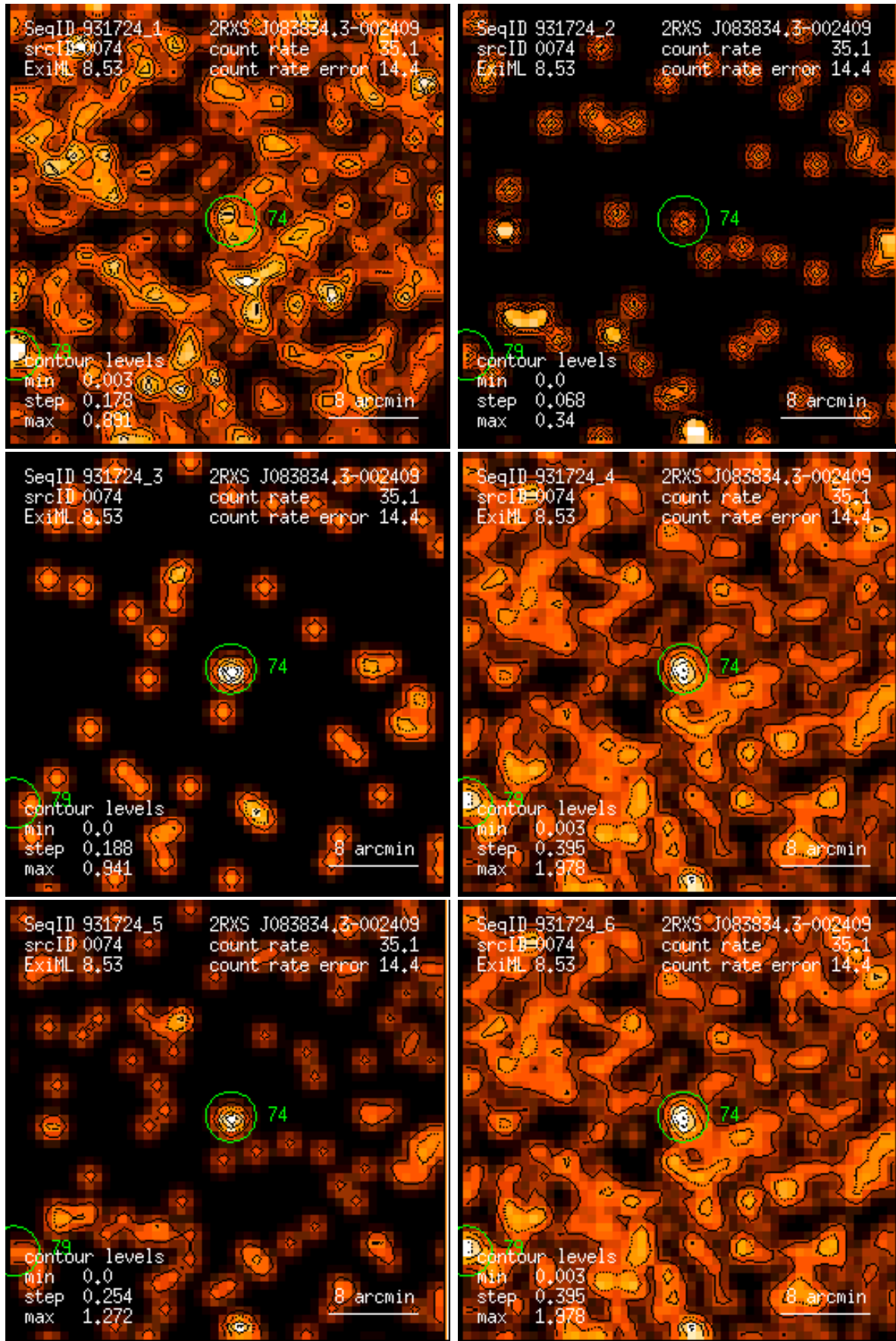
Figure 74: RASS 931724: detection 0074: band rate images, Gaussian filter: (1) PSPC channels 11 – 41, (2) 52 – 90, (3) 91 – 201, (4) 11 – 235, (5) 52 – 201, (6) 11 – 201. Broad band rates in counts/ks. Band rate contour levels in counts/ks/arcmin 2 .
