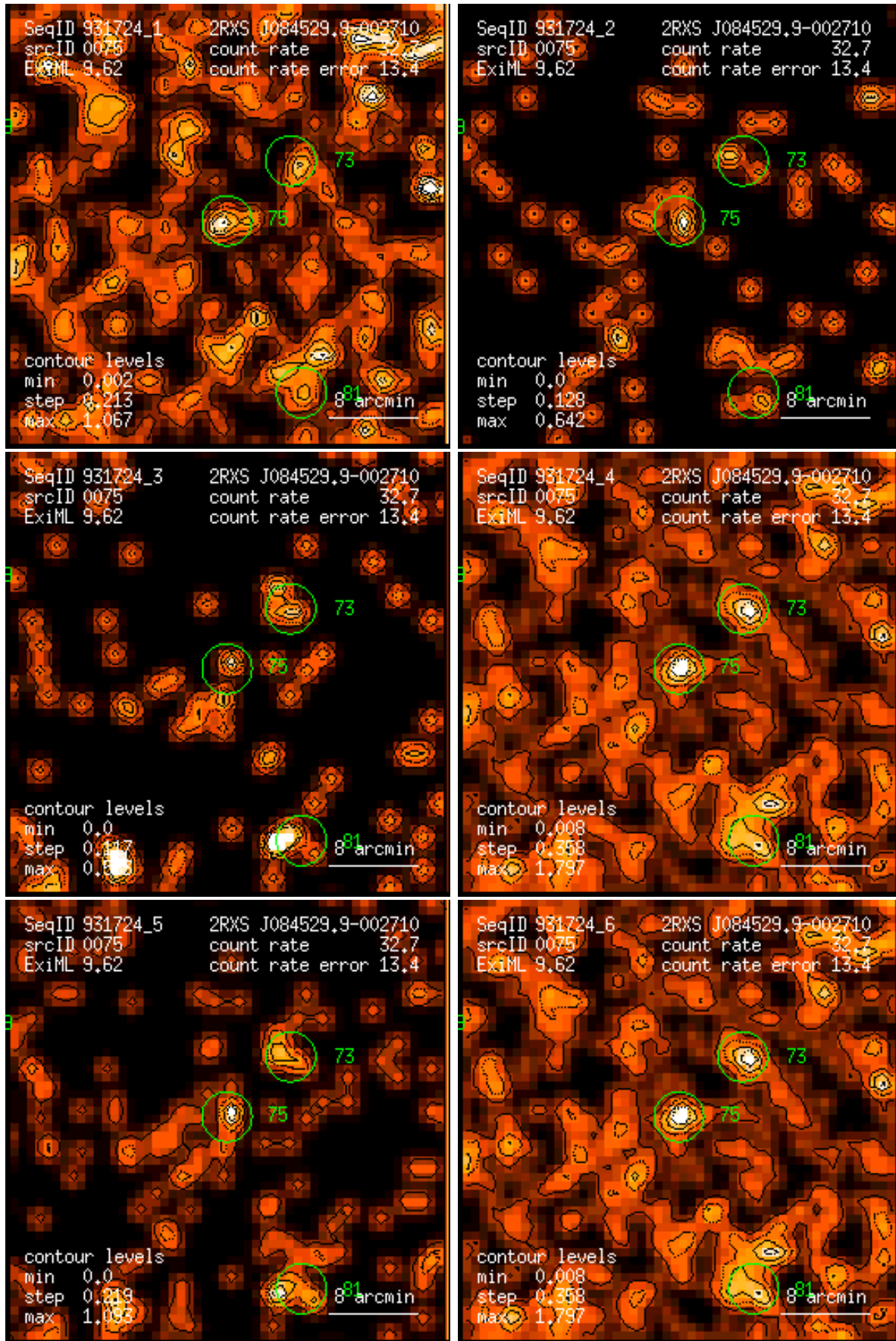
Figure 75: RASS 931724: detection 0075: band rate images, Gaussian filter: (1) PSPC channels 11 – 41, (2) 52 – 90, (3) 91 – 201, (4) 11 – 235, (5) 52 – 201, (6) 11 – 201. Broad band rates in counts/ks. Band rate contour levels in counts/ks/arcmin 2 .
