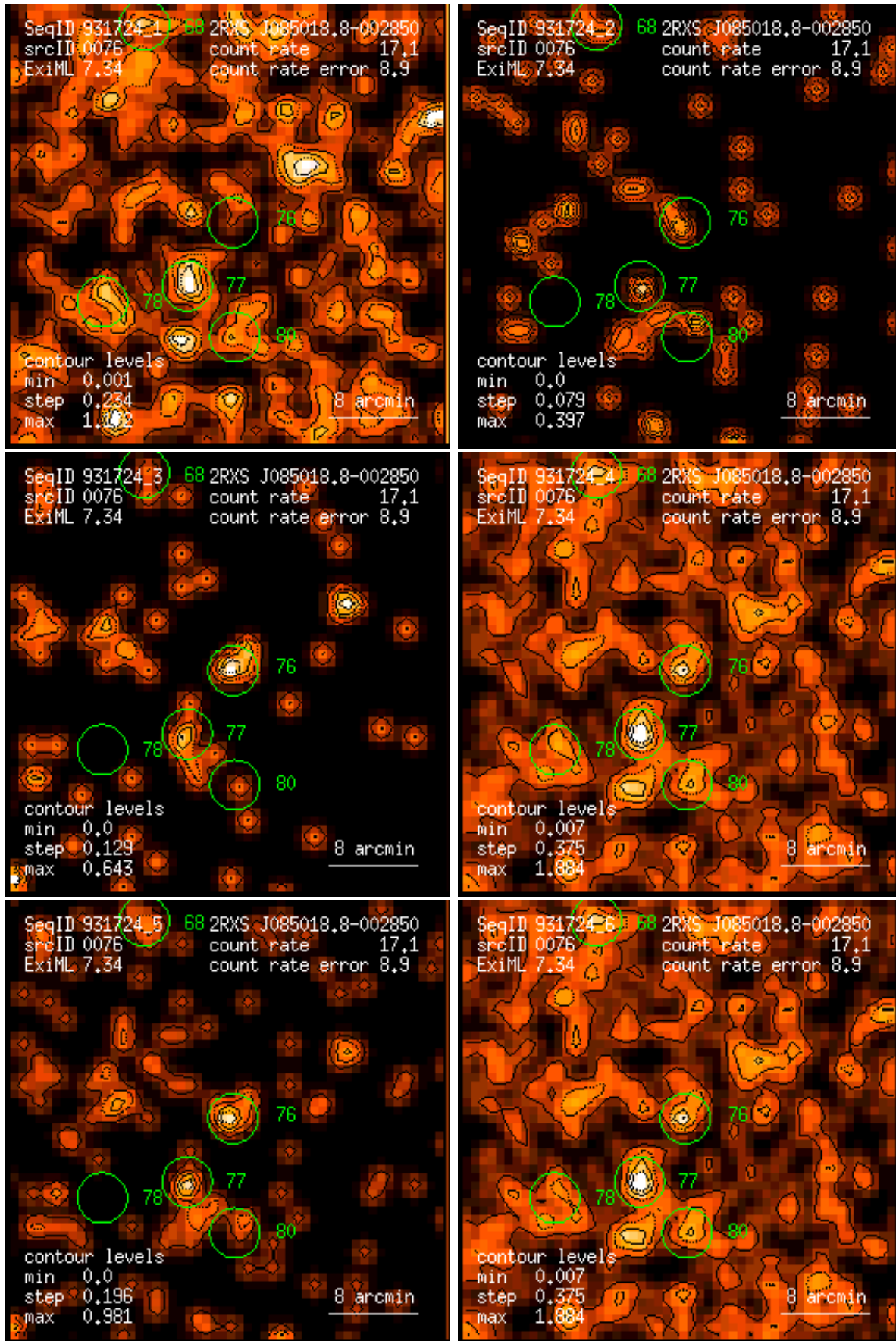
Figure 76: RASS 931724: detection 0076: band rate images, Gaussian filter: (1) PSPC channels 11 – 41, (2) 52 – 90, (3) 91 – 201, (4) 11 – 235, (5) 52 – 201, (6) 11 – 201. Broad band rates in counts/ks. Band rate contour levels in counts/ks/arcmin 2 .
