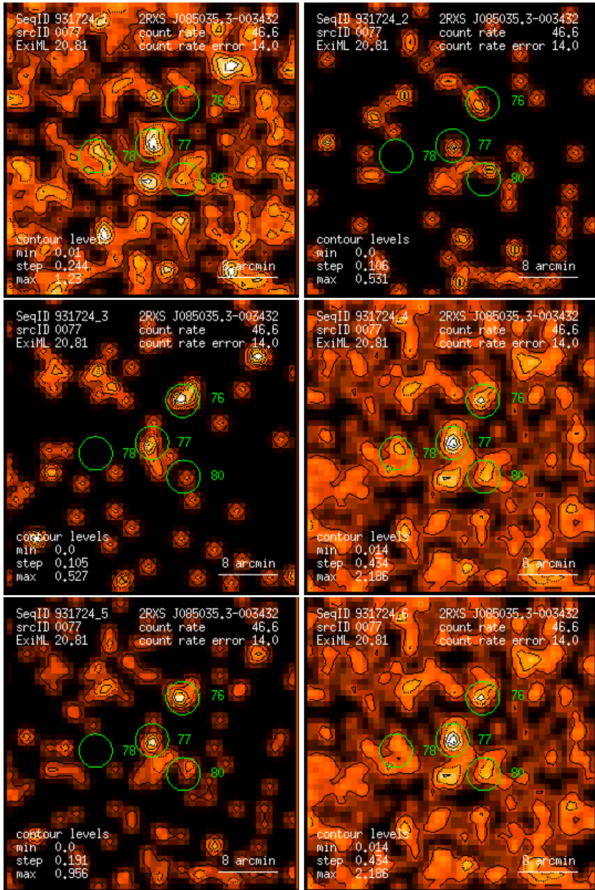
Figure 77: RASS 931724: detection 0077: band rate images, Gaussian filter: (1) PSPC channels 11 – 41, (2) 52 – 90, (3) 91 – 201, (4) 11 – 235, (5) 52 – 201, (6) 11 – 201. Broad band rates in counts/ks. Band rate contour levels in counts/ks/arcmin 2 .
