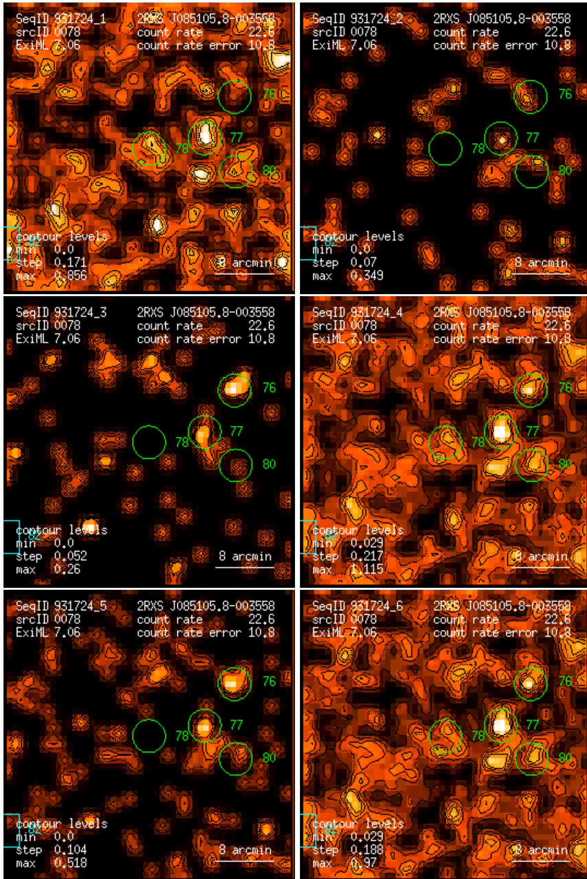
Figure 78: RASS 931724: detection 0078: band rate images, Gaussian filter: (1) PSPC channels 11 – 41, (2) 52 – 90, (3) 91 – 201, (4) 11 – 235, (5) 52 – 201, (6) 11 – 201. Broad band rates in counts/ks. Band rate contour levels in counts/ks/arcmin 2 .
