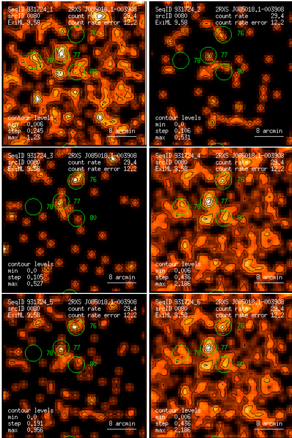
Figure 80: RASS 931724: detection 0080: band rate images, Gaussian filter: (1) PSPC channels 11 – 41, (2) 52 – 90, (3) 91 – 201, (4) 11 – 235, (5) 52 – 201, (6) 11 – 201. Broad band rates in counts/ks. Band rate contour levels in counts/ks/arcmin 2 .
