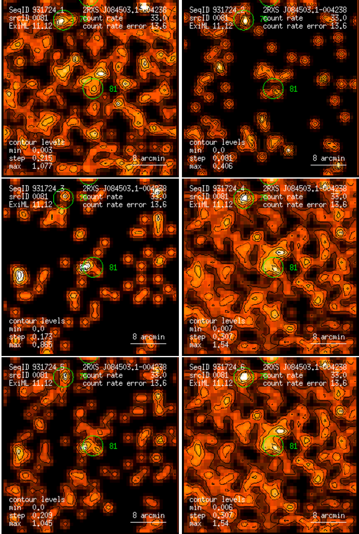
Figure 81: RASS 931724: detection 0081: band rate images, Gaussian filter: (1) PSPC channels 11 – 41, (2) 52 – 90, (3) 91 – 201, (4) 11 – 235, (5) 52 – 201, (6) 11 – 201. Broad band rates in counts/ks. Band rate contour levels in counts/ks/arcmin 2 .
