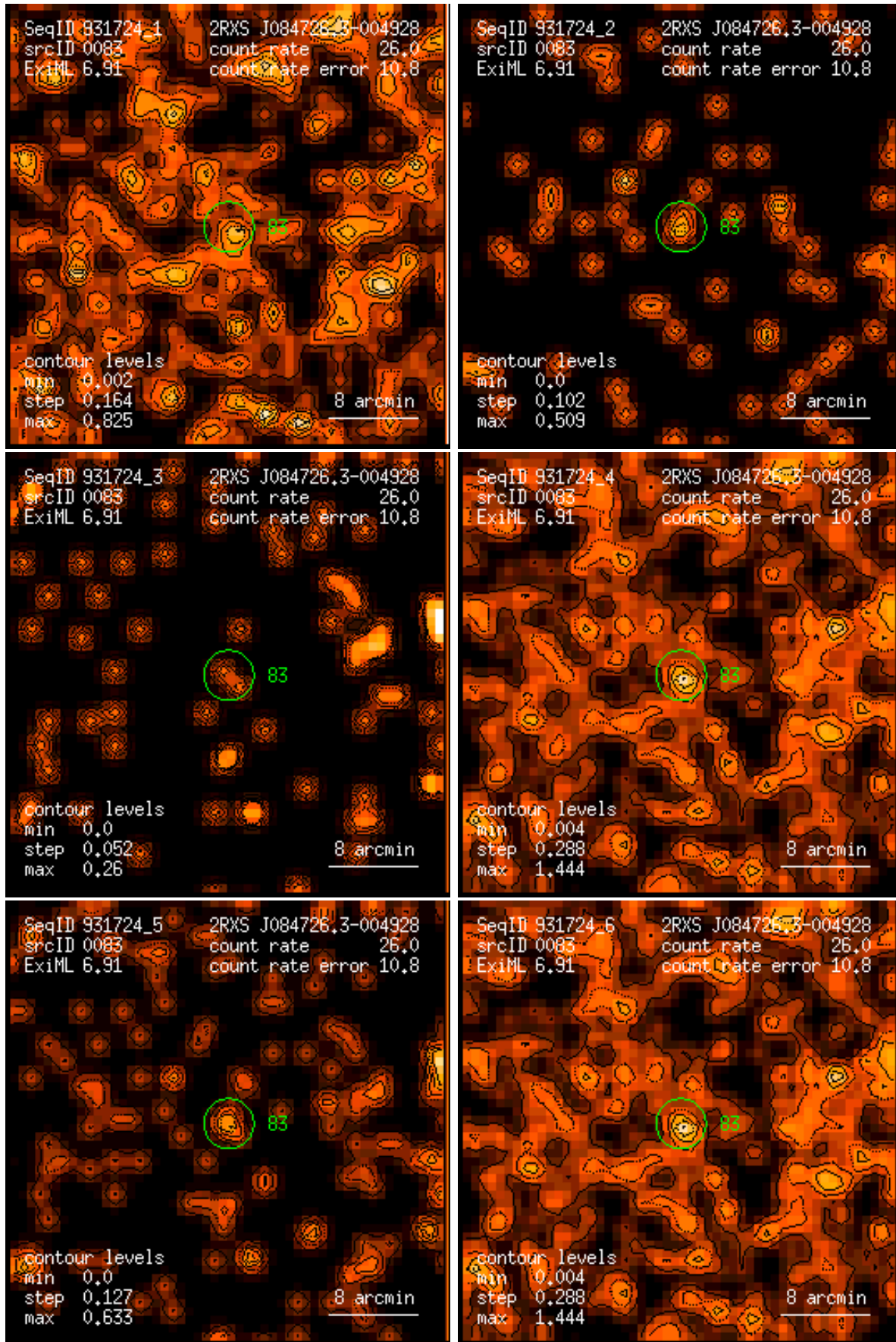
Figure 83: RASS 931724: detection 0083: band rate images, Gaussian filter: (1) PSPC channels 11 – 41, (2) 52 – 90, (3) 91 – 201, (4) 11 – 235, (5) 52 – 201, (6) 11 – 201. Broad band rates in counts/ks. Band rate contour levels in counts/ks/arcmin 2 .
