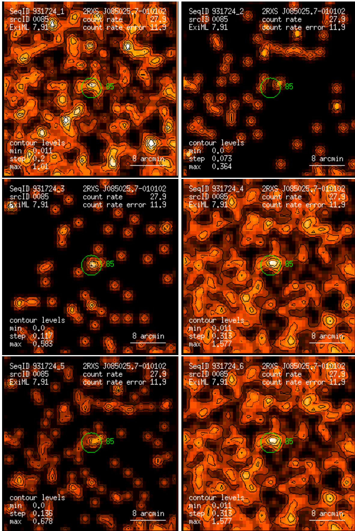
Figure 85: RASS 931724: detection 0085: band rate images, Gaussian filter: (1) PSPC channels 11 – 41, (2) 52 – 90, (3) 91 – 201, (4) 11 – 235, (5) 52 – 201, (6) 11 – 201. Broad band rates in counts/ks. Band rate contour levels in counts/ks/arcmin 2 .
