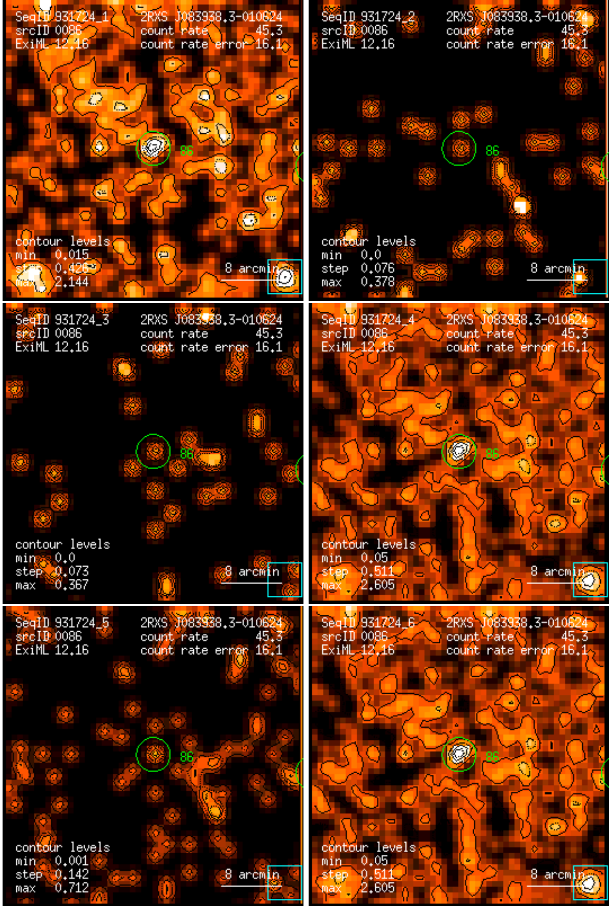
Figure 86: RASS 931724: detection 0086: band rate images, Gaussian filter: (1) PSPC channels 11 – 41, (2) 52 – 90, (3) 91 – 201, (4) 11 – 235, (5) 52 – 201, (6) 11 – 201. Broad band rates in counts/ks. Band rate contour levels in counts/ks/arcmin 2 .
