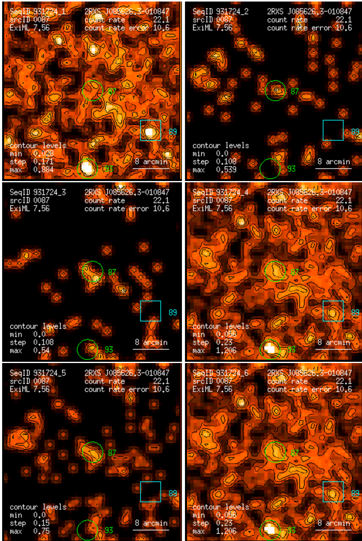
Figure 87: RASS 931724: detection 0087: band rate images, Gaussian filter: (1) PSPC channels 11 – 41, (2) 52 – 90, (3) 91 – 201, (4) 11 – 235, (5) 52 – 201, (6) 11 – 201. Broad band rates in counts/ks. Band rate contour levels in counts/ks/arcmin 2 .
