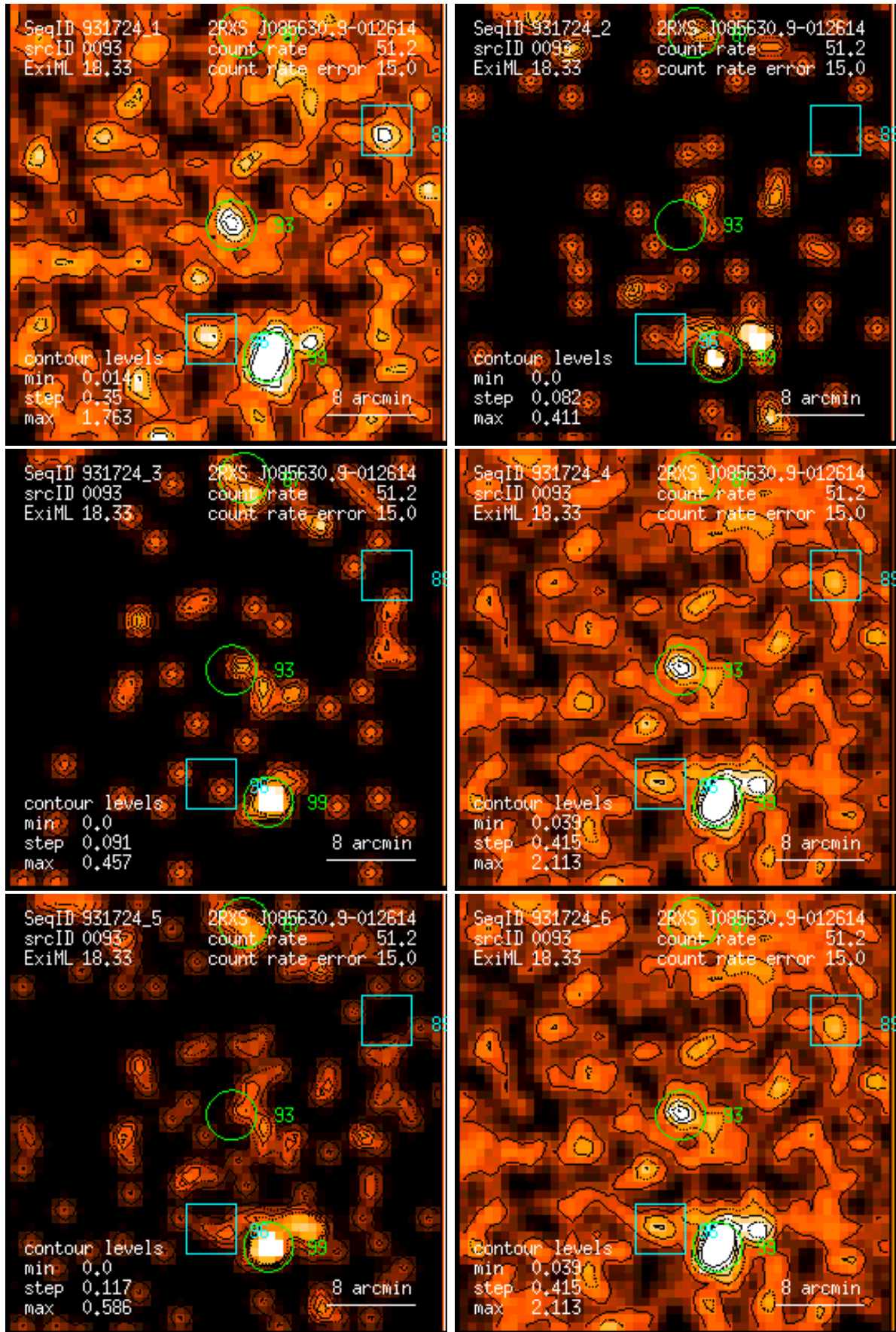
Figure 93: RASS 931724: detection 0093: band rate images, Gaussian filter: (1) PSPC channels 11 – 41, (2) 52 – 90, (3) 91 – 201, (4) 11 – 235, (5) 52 – 201, (6) 11 – 201. Broad band rates in counts/ks. Band rate contour levels in counts/ks/arcmin 2 .
