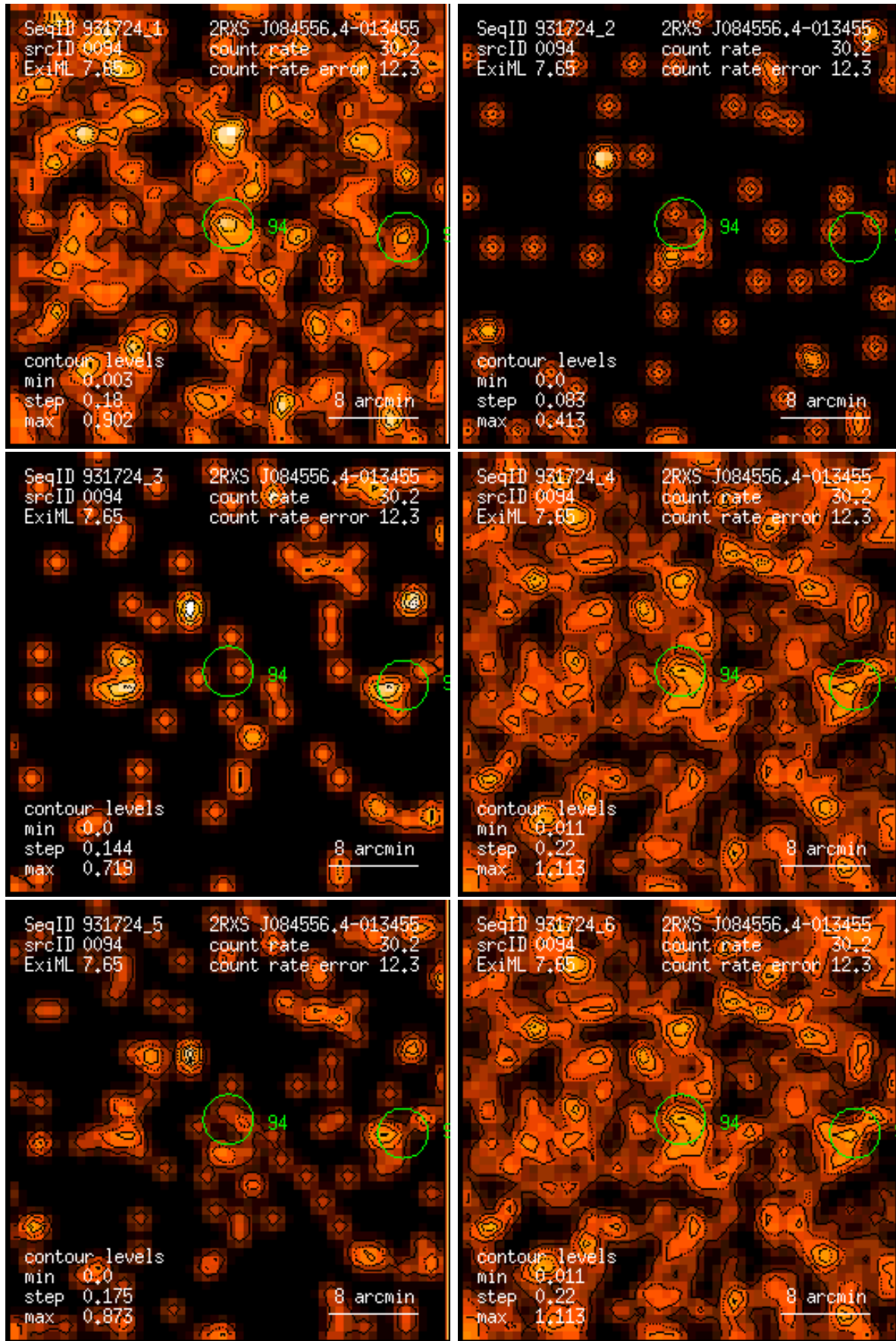
Figure 94: RASS 931724: detection 0094: band rate images, Gaussian filter: (1) PSPC channels 11 – 41, (2) 52 – 90, (3) 91 – 201, (4) 11 – 235, (5) 52 – 201, (6) 11 – 201. Broad band rates in counts/ks. Band rate contour levels in counts/ks/arcmin 2 .
