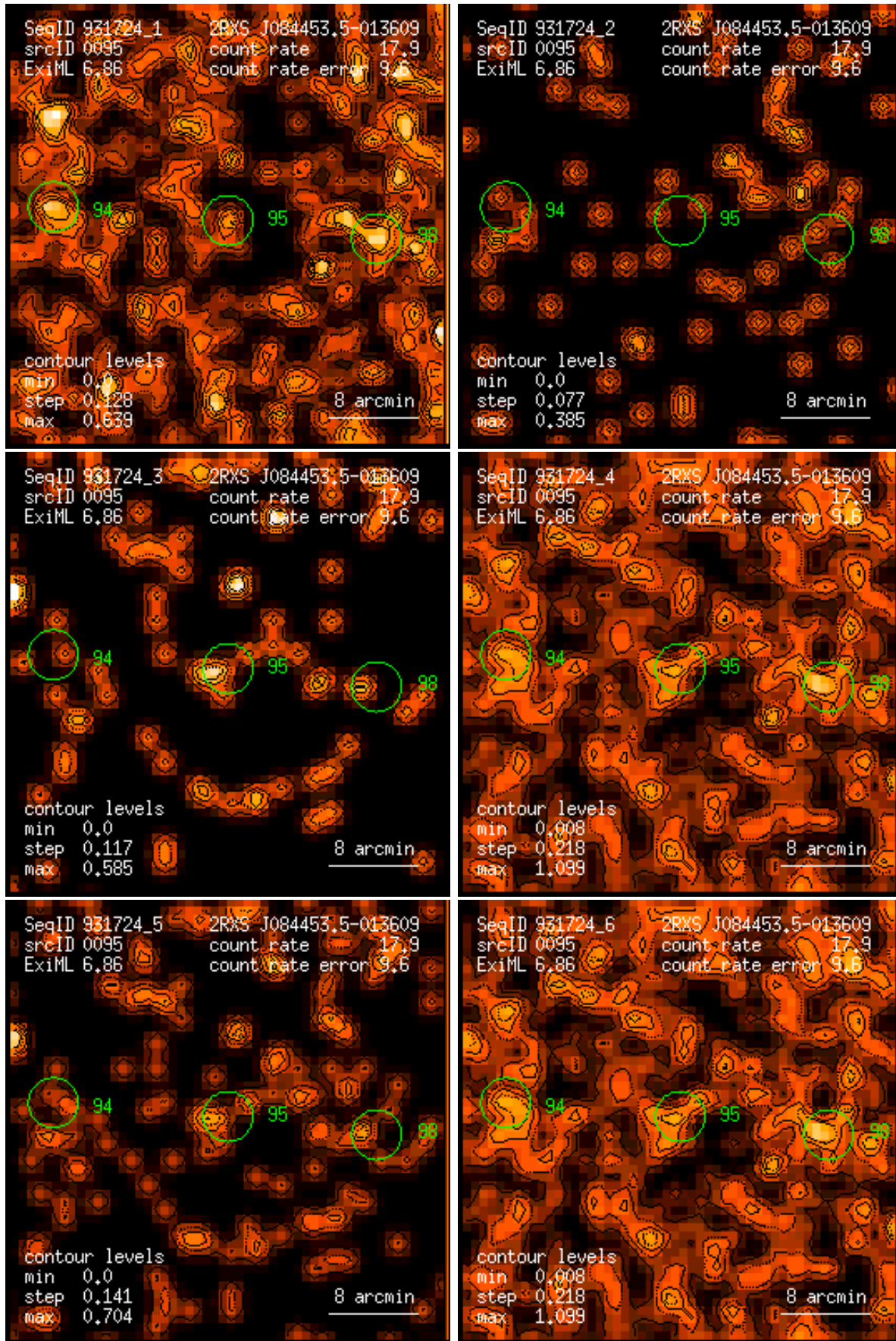
Figure 95: RASS 931724: detection 0095: band rate images, Gaussian filter: (1) PSPC channels 11 – 41, (2) 52 – 90, (3) 91 – 201, (4) 11 – 235, (5) 52 – 201, (6) 11 – 201. Broad band rates in counts/ks. Band rate contour levels in counts/ks/arcmin 2 .
