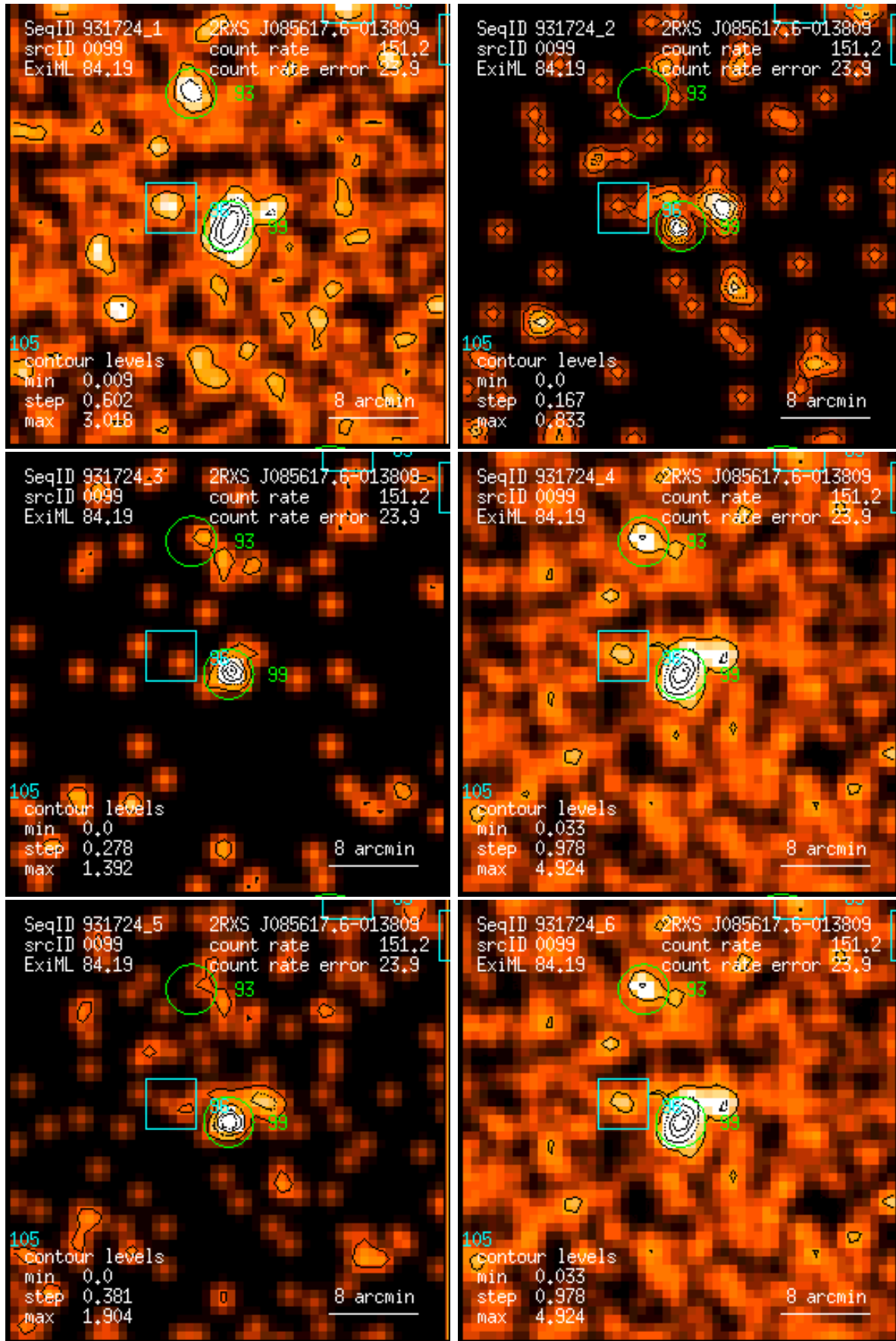
Figure 99: RASS 931724: detection 0099: band rate images, Gaussian filter: (1) PSPC channels 11 – 41, (2) 52 – 90, (3) 91 – 201, (4) 11 – 235, (5) 52 – 201, (6) 11 – 201. Broad band rates in counts/ks. Band rate contour levels in counts/ks/arcmin 2 .
