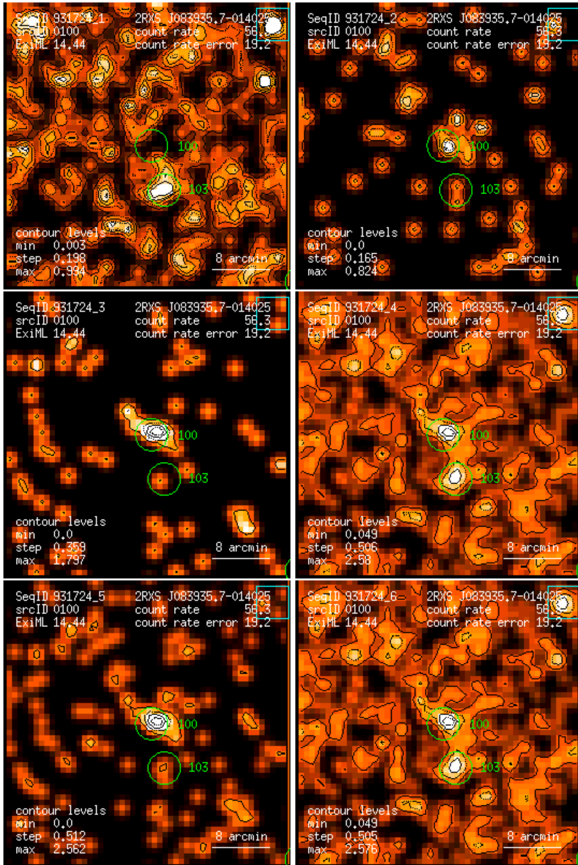
Figure 100: RASS 931724: detection 0100: band rate images, Gaussian filter: (1) PSPC channels 11 – 41, (2) 52 – 90, (3) 91 – 201, (4) 11 – 235, (5) 52 – 201, (6) 11 – 201. Broad band rates in counts/ks. Band rate contour levels in counts/ks/arcmin 2 .
