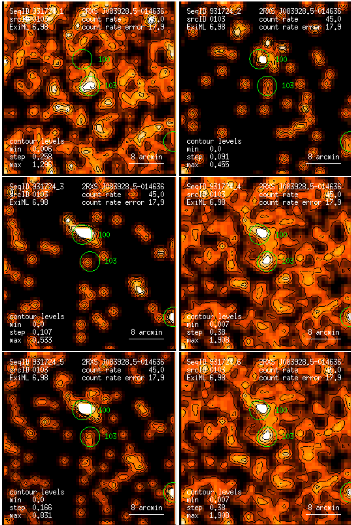
Figure 103: RASS 931724: detection 0103: band rate images, Gaussian filter: (1) PSPC channels 11 – 41, (2) 52 – 90, (3) 91 – 201, (4) 11 – 235, (5) 52 – 201, (6) 11 – 201. Broad band rates in counts/ks. Band rate contour levels in counts/ks/arcmin 2 .
