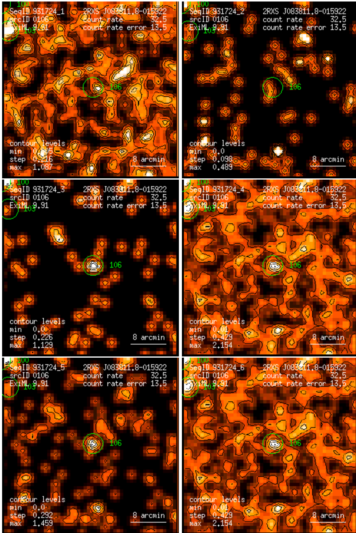
Figure 106: RASS 931724: detection 0106: band rate images, Gaussian filter: (1) PSPC channels 11 – 41, (2) 52 – 90, (3) 91 – 201, (4) 11 – 235, (5) 52 – 201, (6) 11 – 201. Broad band rates in counts/ks. Band rate contour levels in counts/ks/arcmin 2 .
