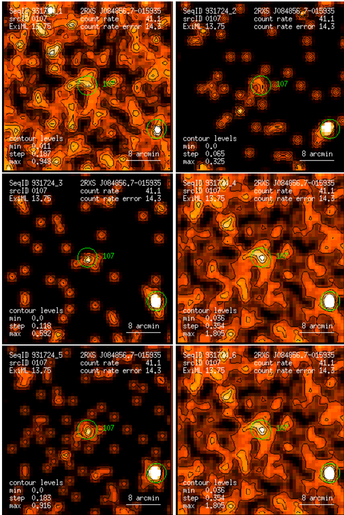
Figure 107: RASS 931724: detection 0107: band rate images, Gaussian filter: (1) PSPC channels 11 – 41, (2) 52 – 90, (3) 91 – 201, (4) 11 – 235, (5) 52 – 201, (6) 11 – 201. Broad band rates in counts/ks. Band rate contour levels in counts/ks/arcmin 2 .
