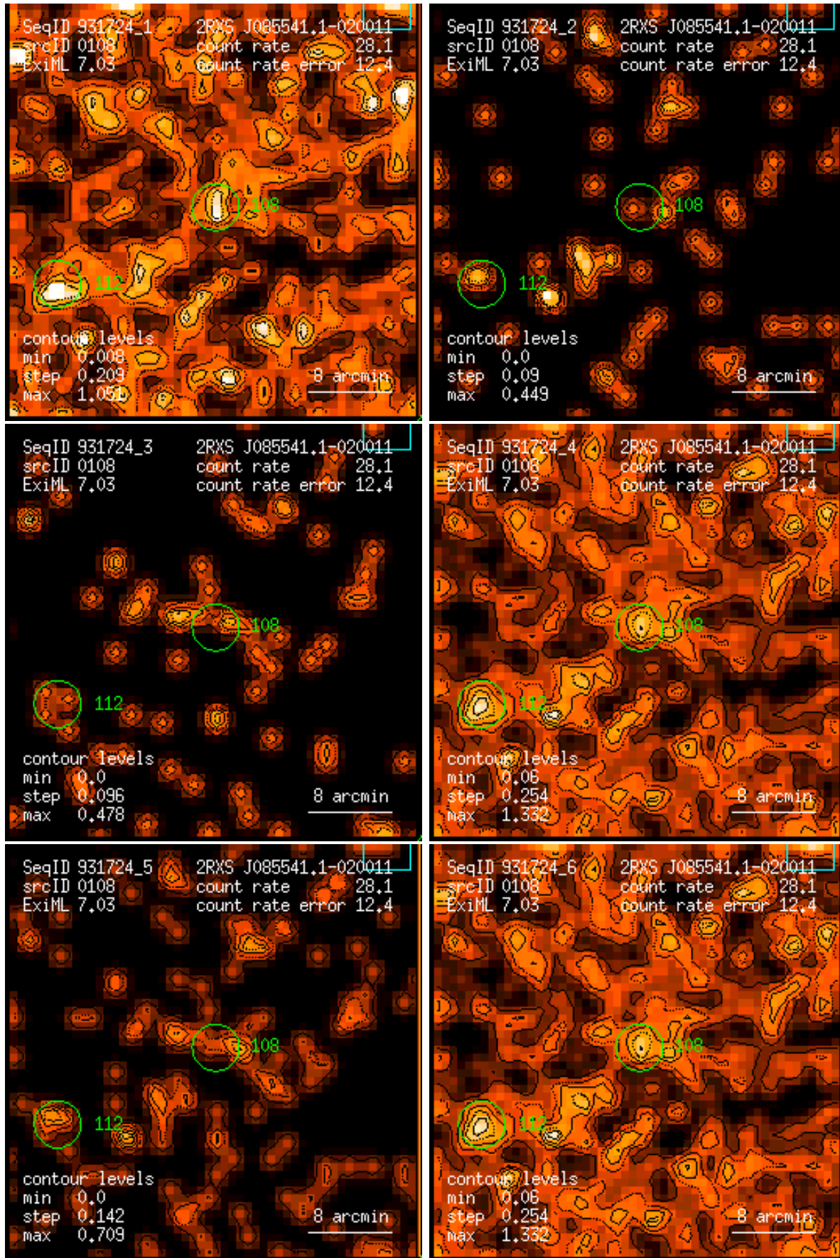
Figure 108: RASS 931724: detection 0108: band rate images, Gaussian filter: (1) PSPC channels 11 – 41, (2) 52 – 90, (3) 91 – 201, (4) 11 – 235, (5) 52 – 201, (6) 11 – 201. Broad band rates in counts/ks. Band rate contour levels in counts/ks/arcmin 2 .
