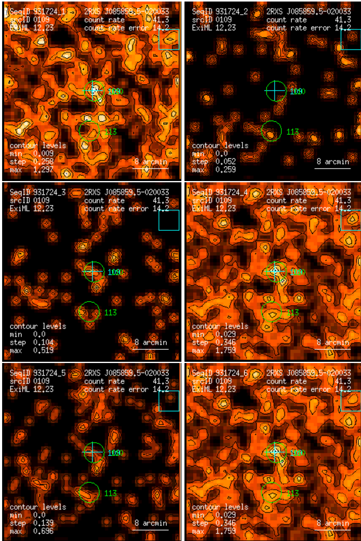
Figure 109: RASS 931724: detection 0109: band rate images, Gaussian filter: (1) PSPC channels 11 – 41, (2) 52 – 90, (3) 91 – 201, (4) 11 – 235, (5) 52 – 201, (6) 11 – 201. Broad band rates in counts/ks. Band rate contour levels in counts/ks/arcmin 2 .
