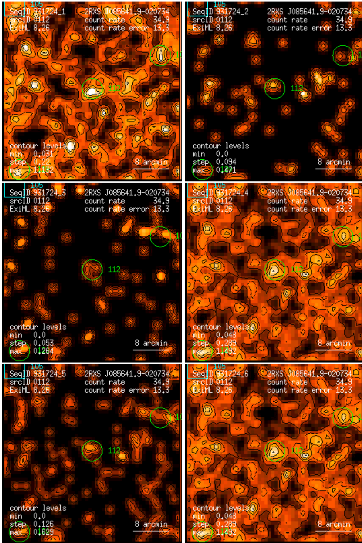
Figure 112: RASS 931724: detection 0112: band rate images, Gaussian filter: (1) PSPC channels 11 – 41, (2) 52 – 90, (3) 91 – 201, (4) 11 – 235, (5) 52 – 201, (6) 11 – 201. Broad band rates in counts/ks. Band rate contour levels in counts/ks/arcmin 2 .
