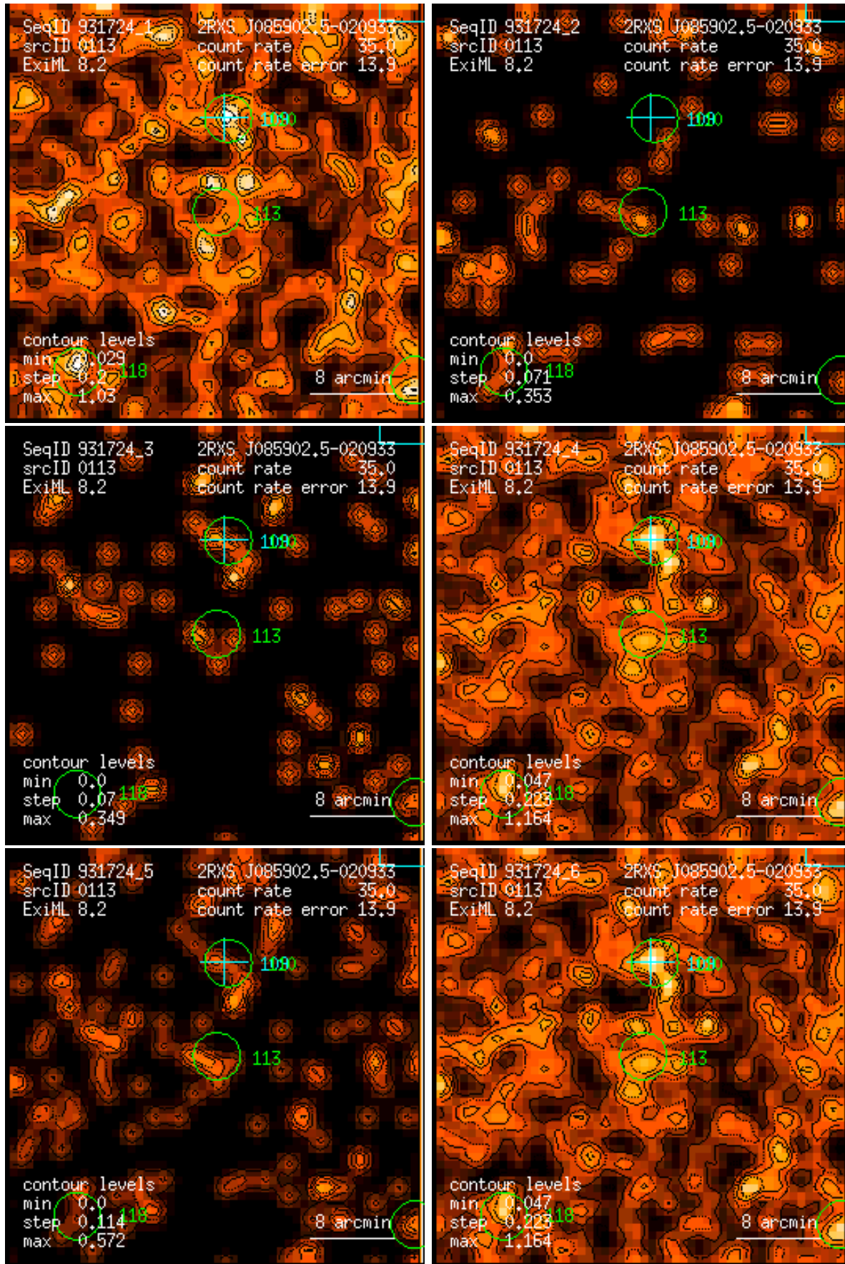
Figure 113: RASS 931724: detection 0113: band rate images, Gaussian filter: (1) PSPC channels 11 – 41, (2) 52 – 90, (3) 91 – 201, (4) 11 – 235, (5) 52 – 201, (6) 11 – 201. Broad band rates in counts/ks. Band rate contour levels in counts/ks/arcmin 2 .
