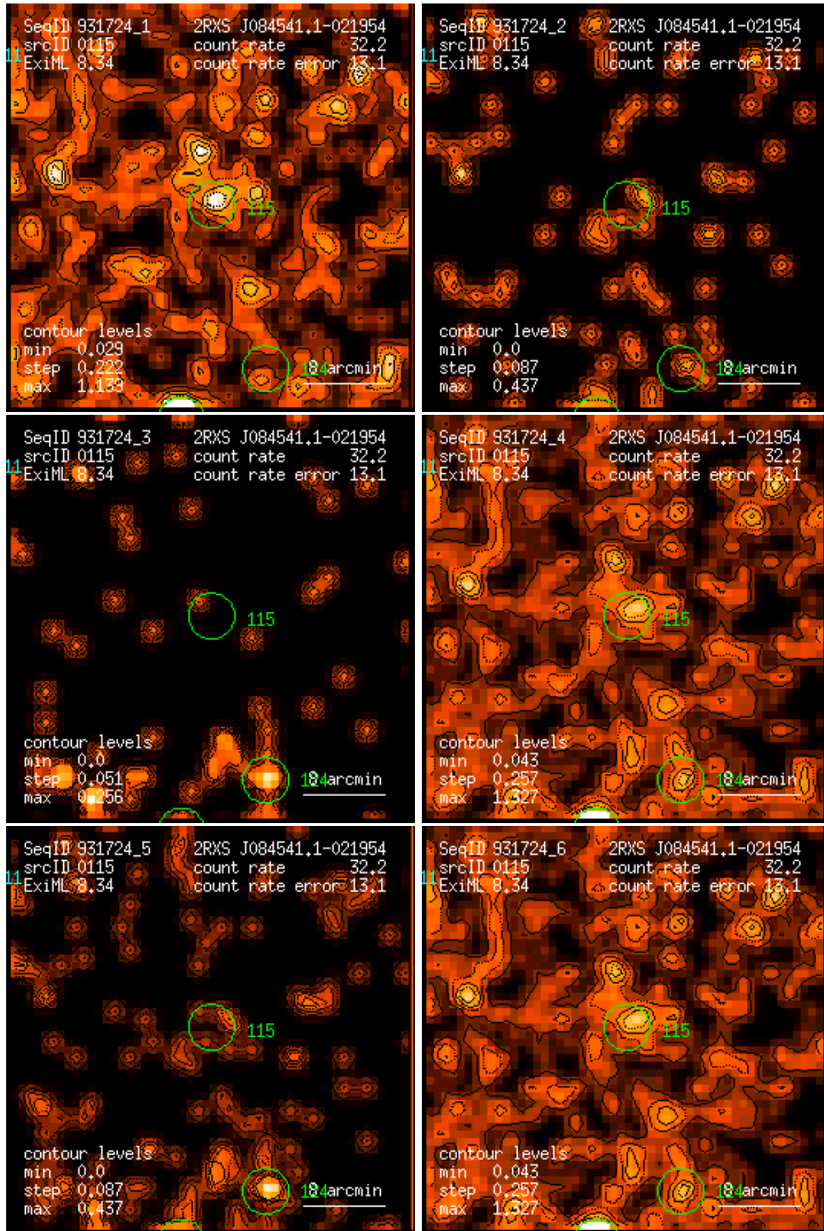
Figure 115: RASS 931724: detection 0115: band rate images, Gaussian filter: (1) PSPC channels 11 – 41, (2) 52 – 90, (3) 91 – 201, (4) 11 – 235, (5) 52 – 201, (6) 11 – 201. Broad band rates in counts/ks. Band rate contour levels in counts/ks/arcmin 2 .
