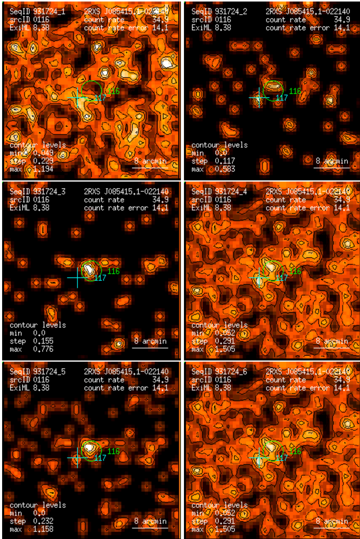
Figure 116: RASS 931724: detection 0116: band rate images, Gaussian filter: (1) PSPC channels 11 – 41, (2) 52 – 90, (3) 91 – 201, (4) 11 – 235, (5) 52 – 201, (6) 11 – 201. Broad band rates in counts/ks. Band rate contour levels in counts/ks/arcmin 2 .
