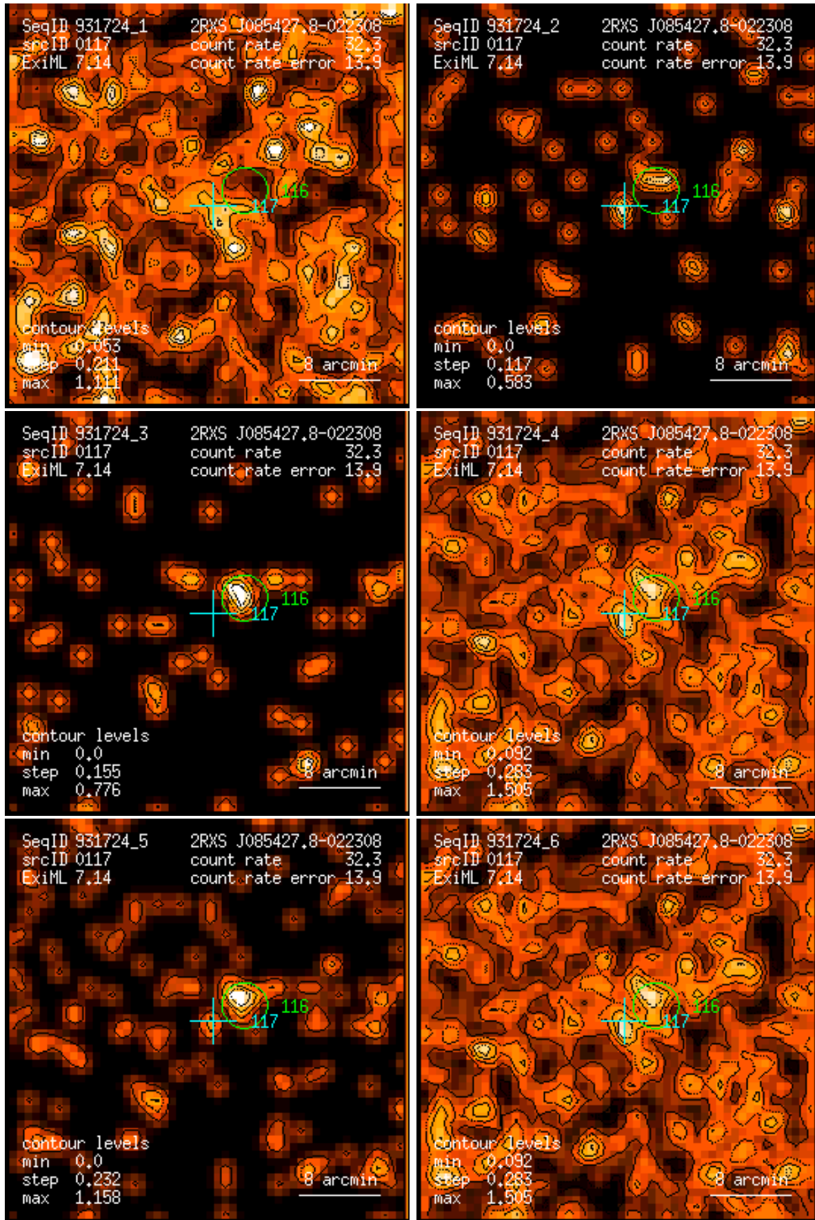
Figure 117: RASS 931724: detection 0117: band rate images, Gaussian filter: (1) PSPC channels 11 – 41, (2) 52 – 90, (3) 91 – 201, (4) 11 – 235, (5) 52 – 201, (6) 11 – 201. Broad band rates in counts/ks. Band rate contour levels in counts/ks/arcmin 2 .
