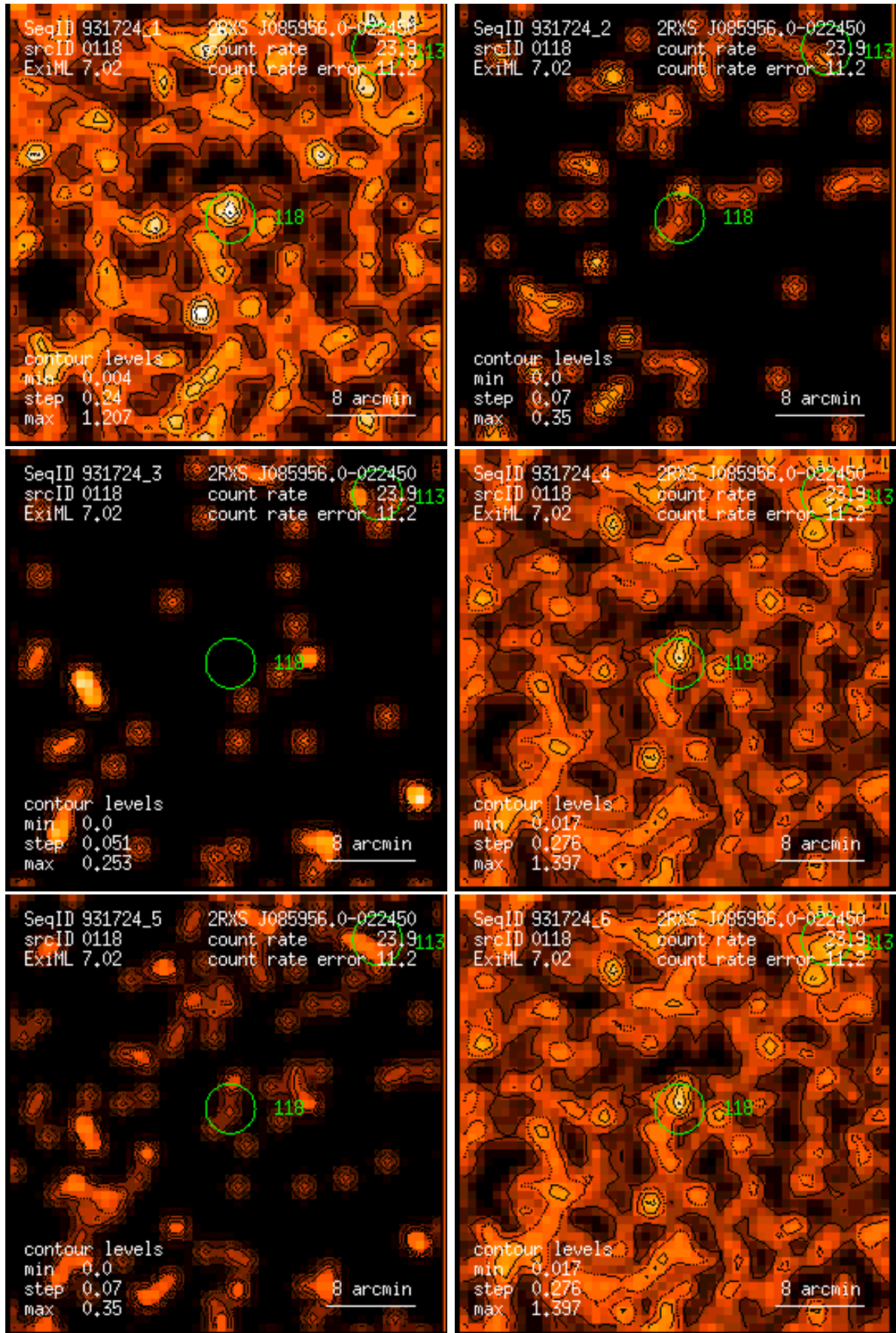
Figure 118: RASS 931724: detection 0118: band rate images, Gaussian filter: (1) PSPC channels 11 – 41, (2) 52 – 90, (3) 91 – 201, (4) 11 – 235, (5) 52 – 201, (6) 11 – 201. Broad band rates in counts/ks. Band rate contour levels in counts/ks/arcmin 2 .
