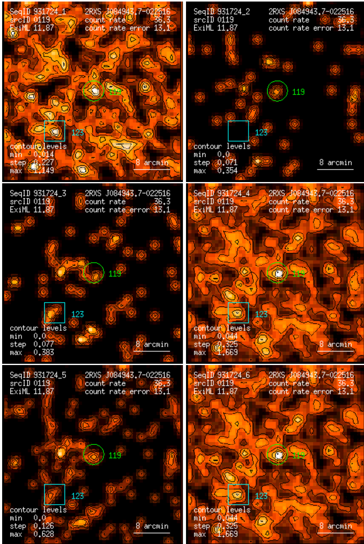
Figure 119: RASS 931724: detection 0119: band rate images, Gaussian filter: (1) PSPC channels 11 – 41, (2) 52 – 90, (3) 91 – 201, (4) 11 – 235, (5) 52 – 201, (6) 11 – 201. Broad band rates in counts/ks. Band rate contour levels in counts/ks/arcmin 2 .
