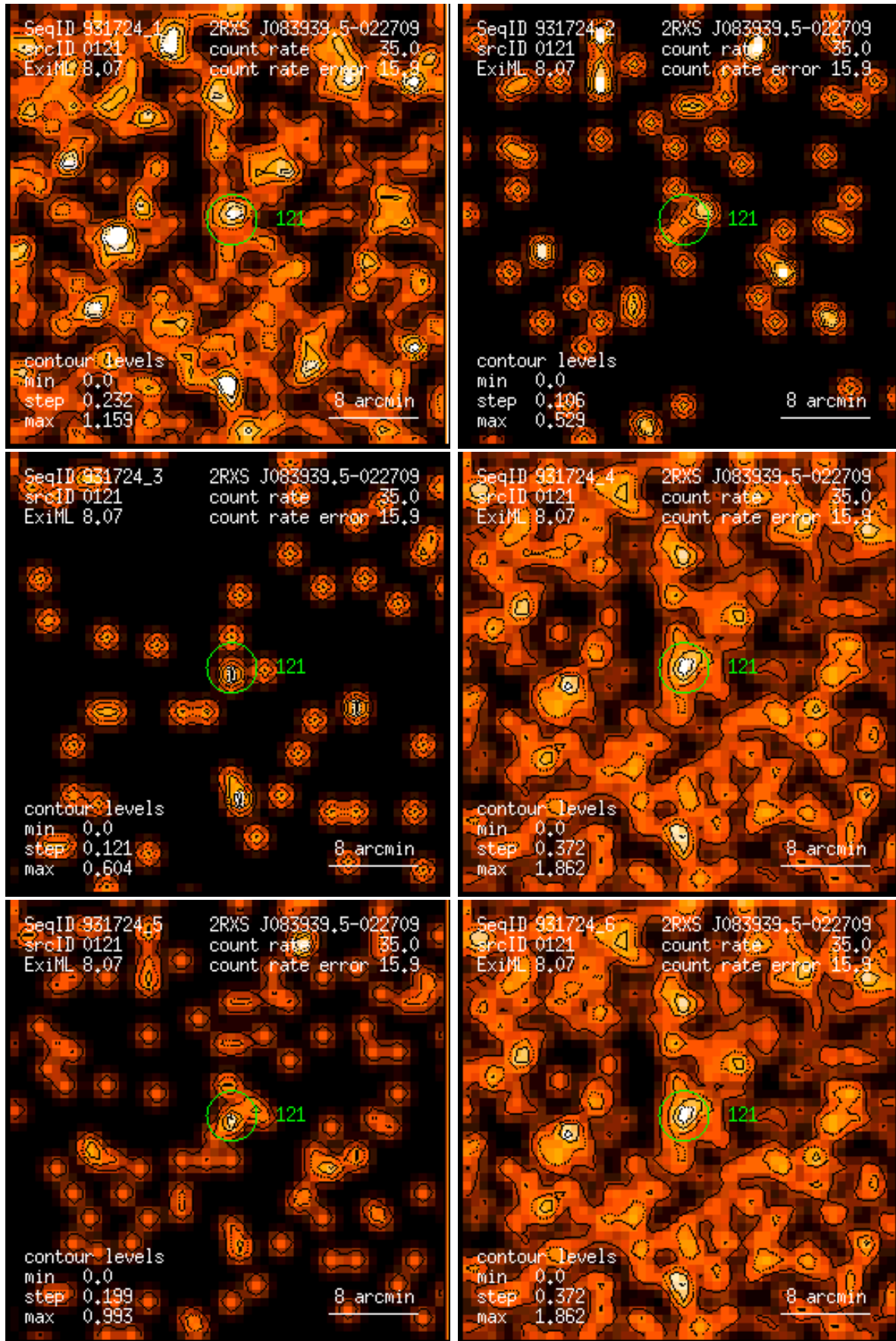
Figure 121: RASS 931724: detection 0121: band rate images, Gaussian filter: (1) PSPC channels 11 – 41, (2) 52 – 90, (3) 91 – 201, (4) 11 – 235, (5) 52 – 201, (6) 11 – 201. Broad band rates in counts/ks. Band rate contour levels in counts/ks/arcmin 2 .
