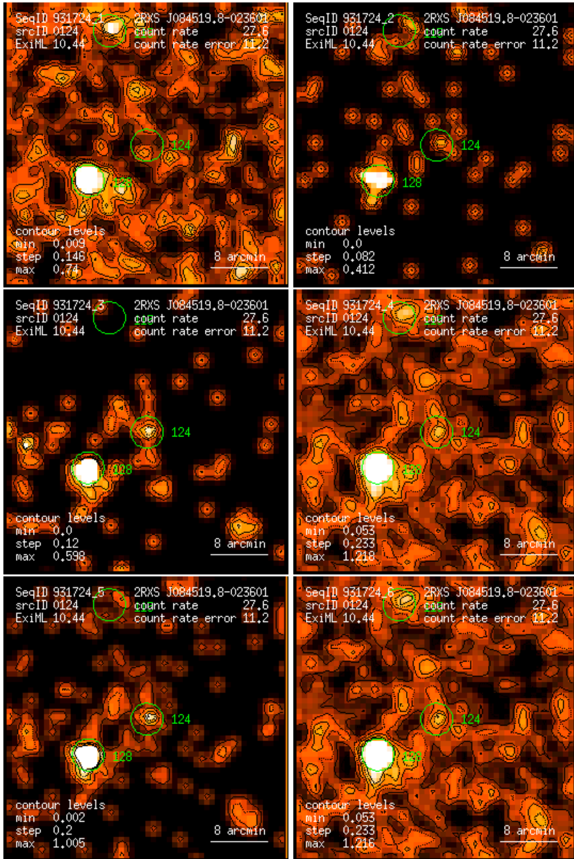
Figure 124: RASS 931724: detection 0124: band rate images, Gaussian filter: (1) PSPC channels 11 – 41, (2) 52 – 90, (3) 91 – 201, (4) 11 – 235, (5) 52 – 201, (6) 11 – 201. Broad band rates in counts/ks. Band rate contour levels in counts/ks/arcmin 2 .
