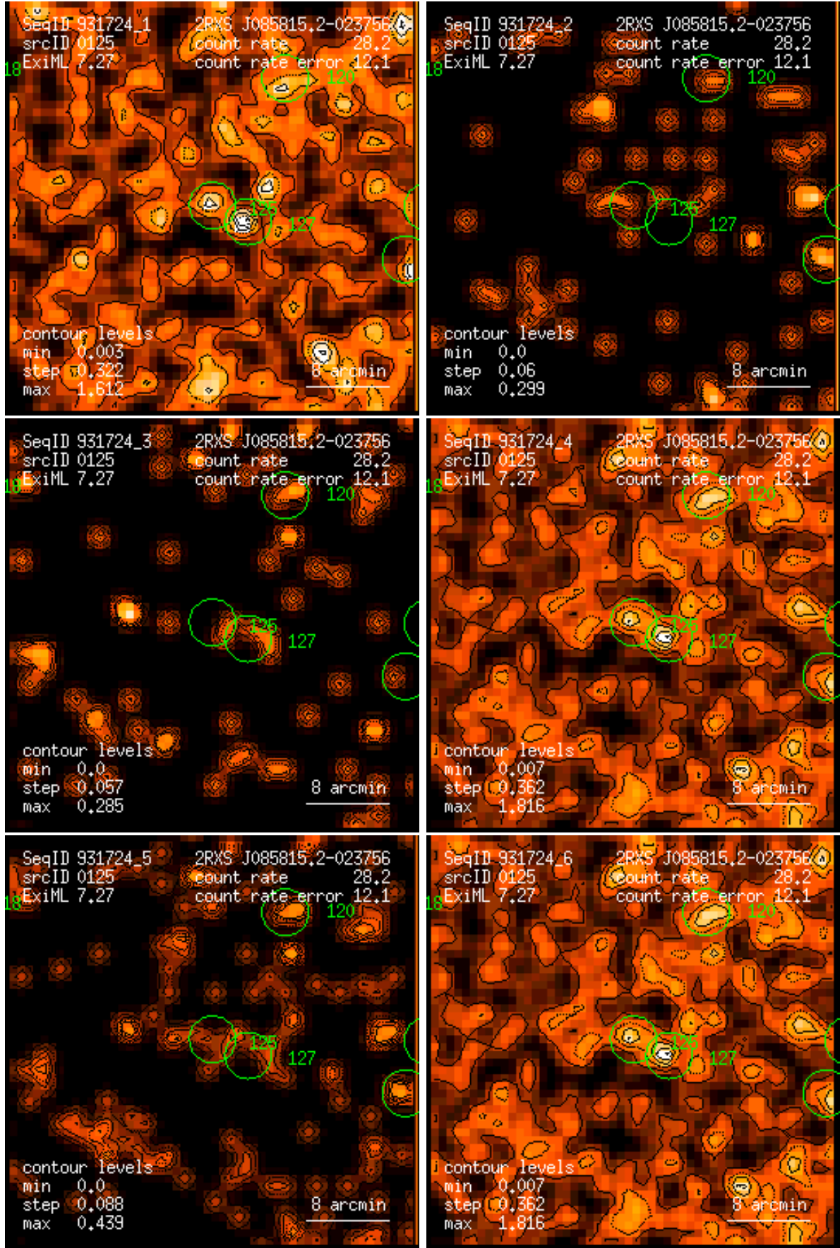
Figure 125: RASS 931724: detection 0125: band rate images, Gaussian filter: (1) PSPC channels 11 – 41, (2) 52 – 90, (3) 91 – 201, (4) 11 – 235, (5) 52 – 201, (6) 11 – 201. Broad band rates in counts/ks. Band rate contour levels in counts/ks/arcmin 2 .
