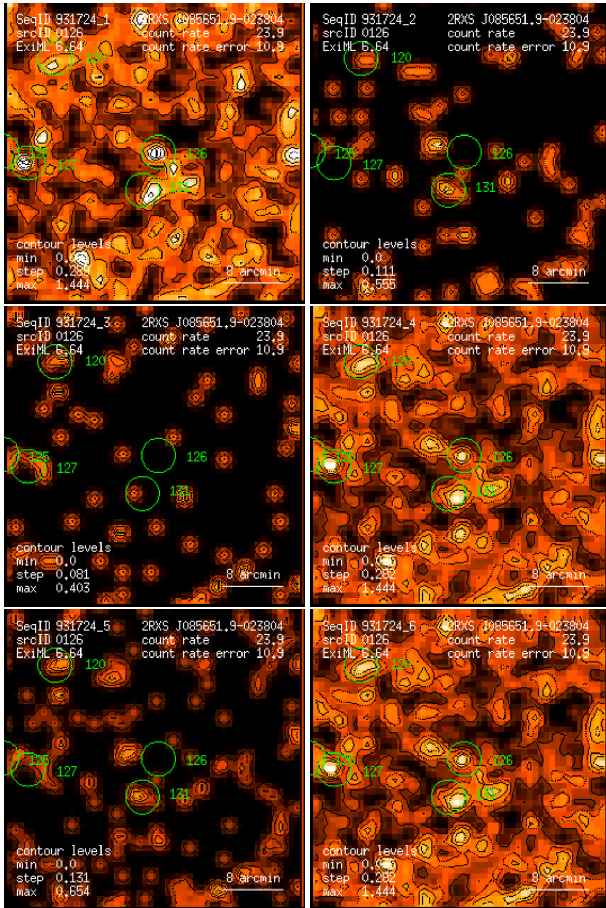
Figure 126: RASS 931724: detection 0126: band rate images, Gaussian filter: (1) PSPC channels 11 – 41, (2) 52 – 90, (3) 91 – 201, (4) 11 – 235, (5) 52 – 201, (6) 11 – 201. Broad band rates in counts/ks. Band rate contour levels in counts/ks/arcmin 2 .
