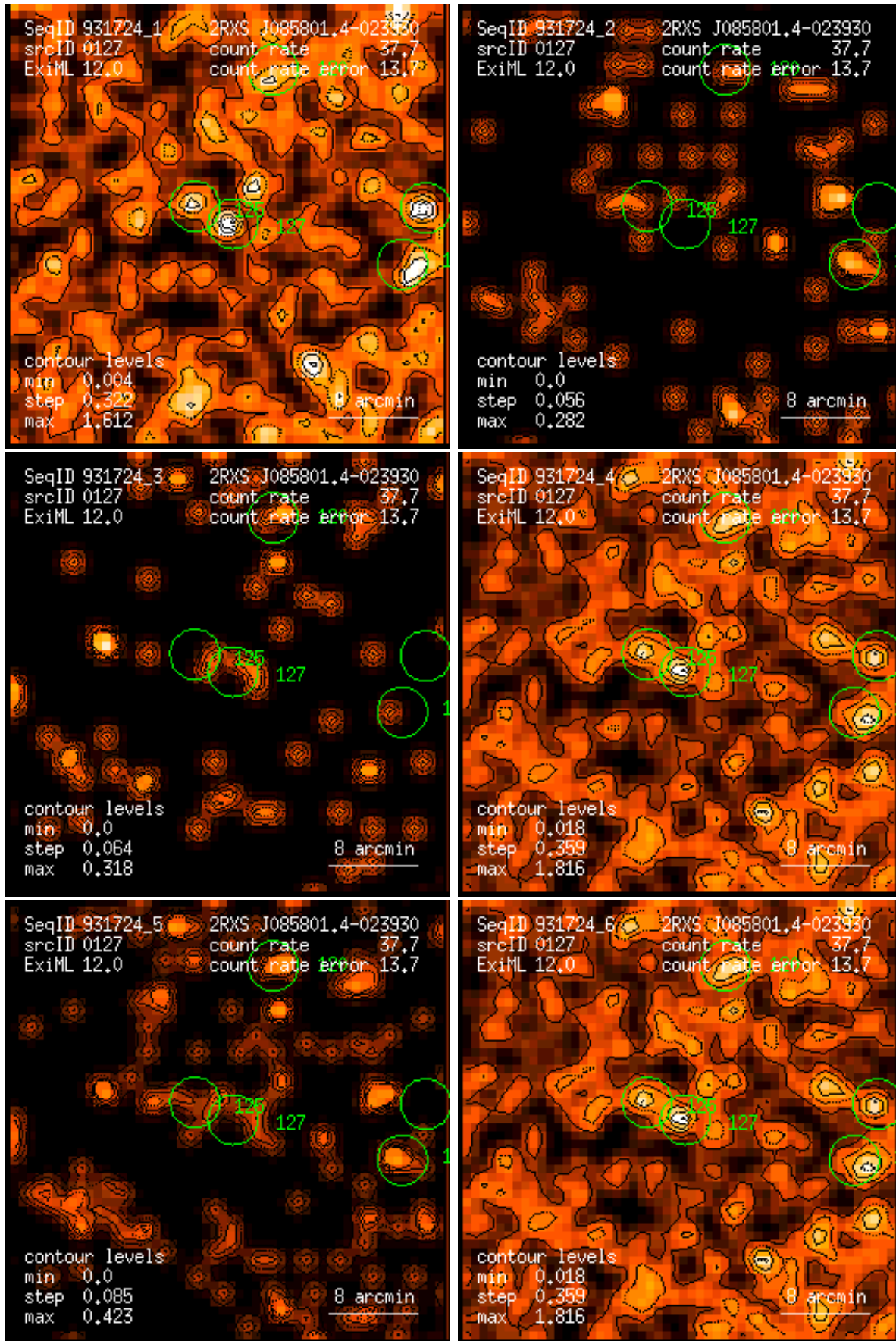
Figure 127: RASS 931724: detection 0127: band rate images, Gaussian filter: (1) PSPC channels 11 – 41, (2) 52 – 90, (3) 91 – 201, (4) 11 – 235, (5) 52 – 201, (6) 11 – 201. Broad band rates in counts/ks. Band rate contour levels in \text{counts/ks/arcmin}^2 .
