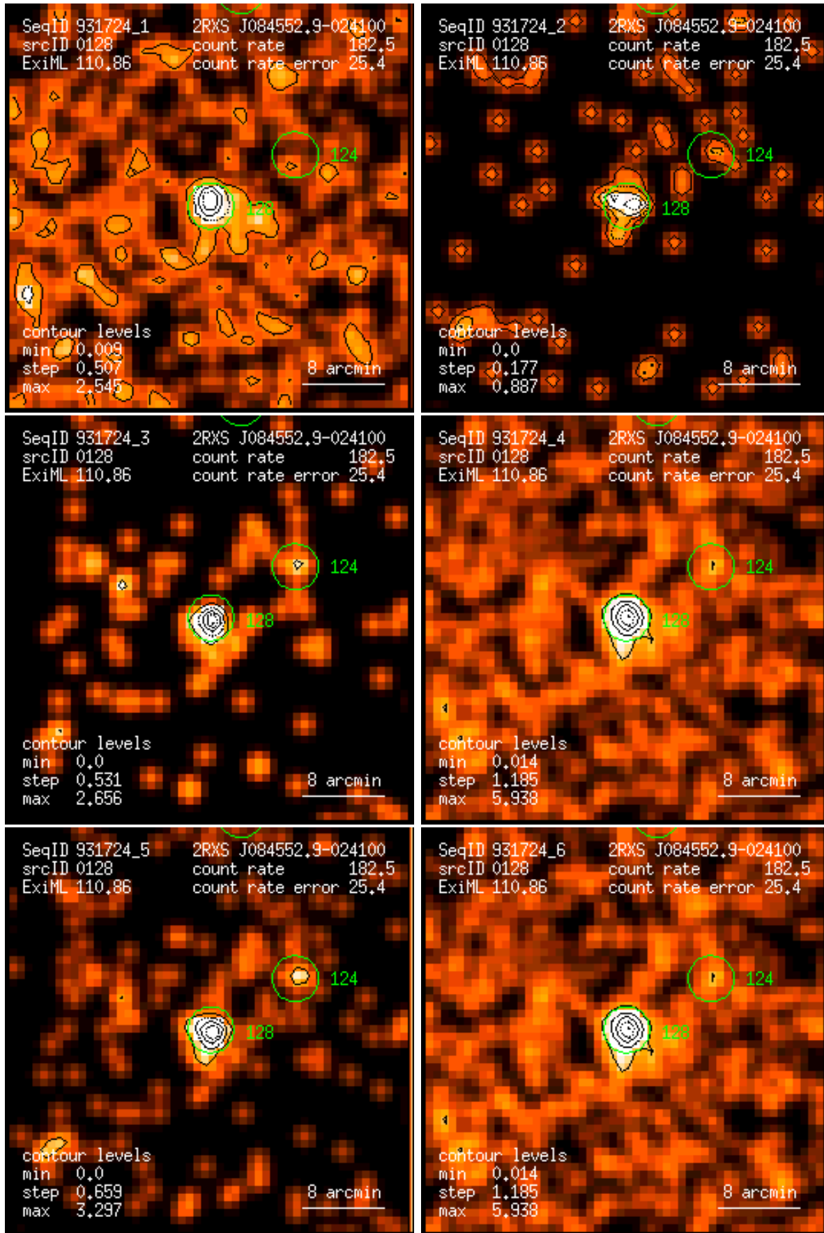
Figure 128: RASS 931724: detection 0128: band rate images, Gaussian filter: (1) PSPC channels 11 – 41, (2) 52 – 90, (3) 91 – 201, (4) 11 – 235, (5) 52 – 201, (6) 11 – 201. Broad band rates in counts/ks. Band rate contour levels in counts/ks/arcmin 2 .
